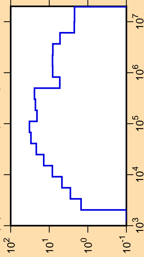
\Delta\mu/\mu vs. E for ^{71}\text{Zn}(\text{mt251})
