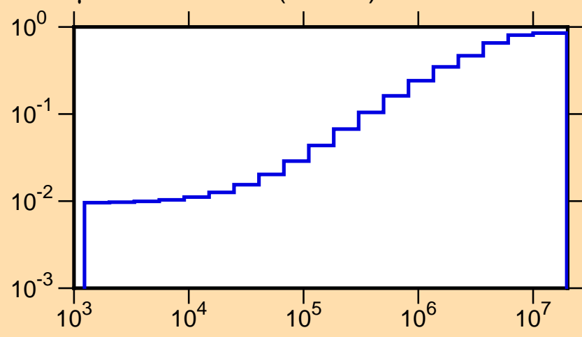
\mu vs. E for ^{71}\text{Zn}(\text{mt251})
