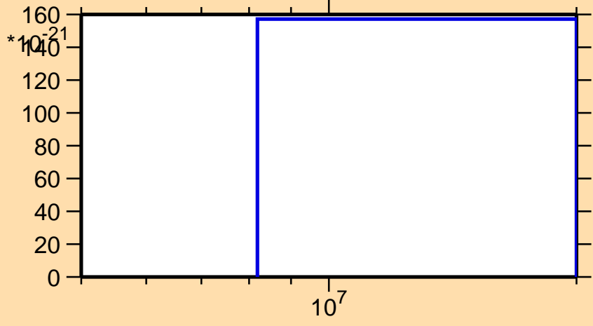
\sigma vs. E for ^{71}\text{Zn}(\text{mt } 34)
