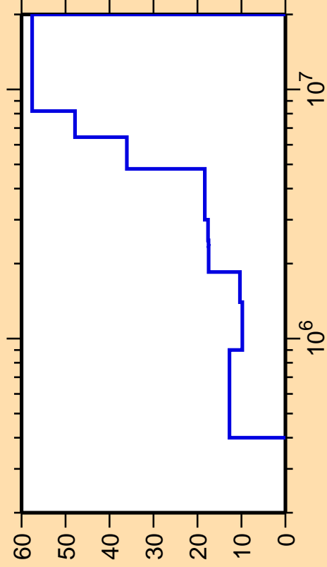
\Delta\sigma/\sigma vs. E for ^{71}\text{Zn}(n,n_3)
