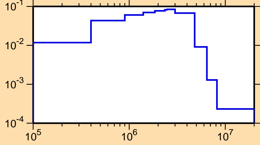
\sigma vs. E for ^{71}\text{Zn}(n,n_1)
