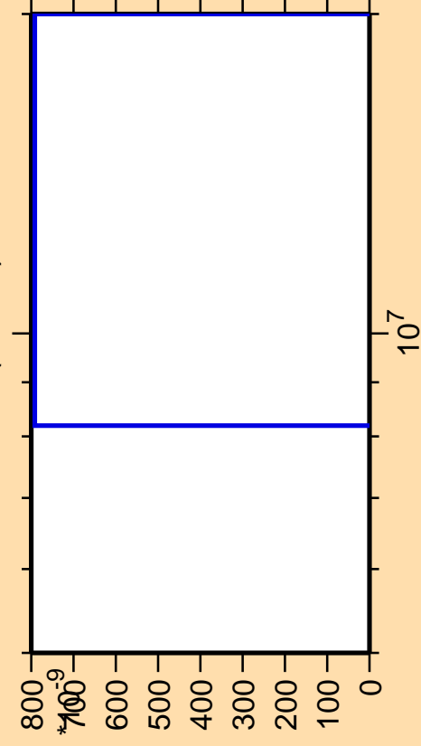
\Delta\sigma/\sigma vs. E for ^{71}\text{Zn}(\text{mt } 34)
