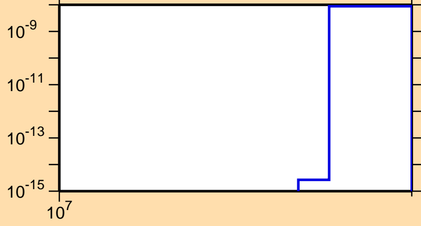
\sigma vs. E for ^{71}\text{Zn}(n,nt)
