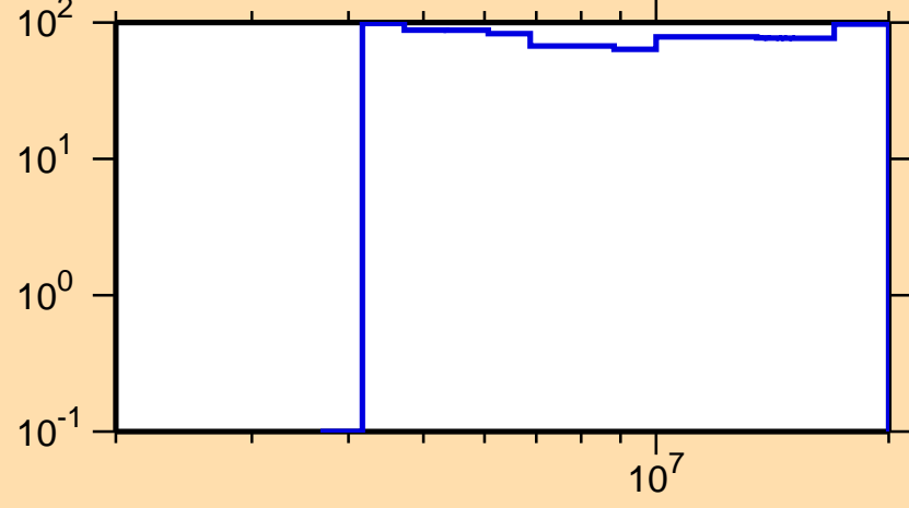
\Delta\sigma/\sigma vs. E for ^{71}\text{Zn}(n,p)
