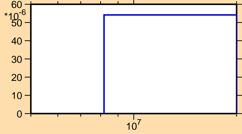
\sigma vs. E for ^{71}\text{Zn}(n,t)
