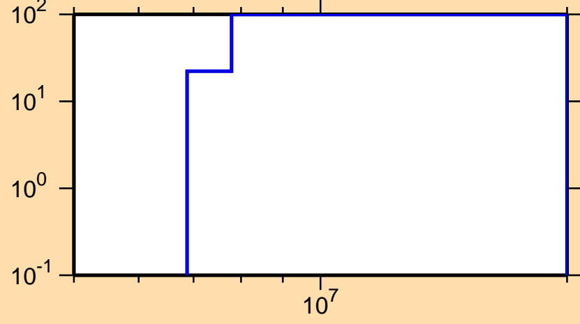
\Delta\sigma/\sigma vs. E for ^{72}\text{Zn}(n,p)
