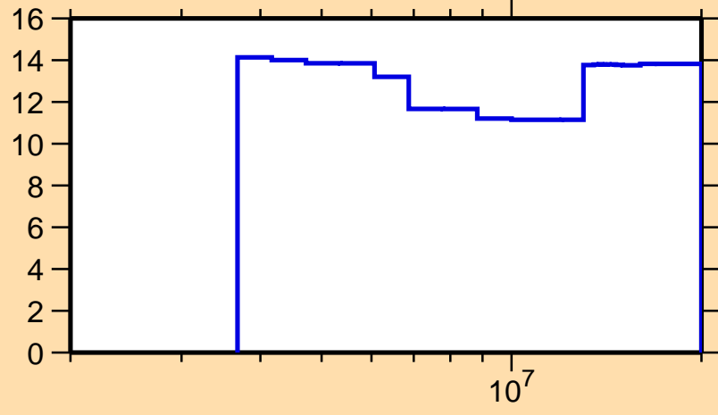
\Delta\sigma/\sigma vs. E for ^{72}\text{Zn}(n,n\text{onel.})
