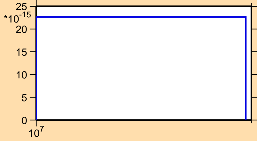
\sigma vs. E for ^{72}\text{Zn}(n,nd)
