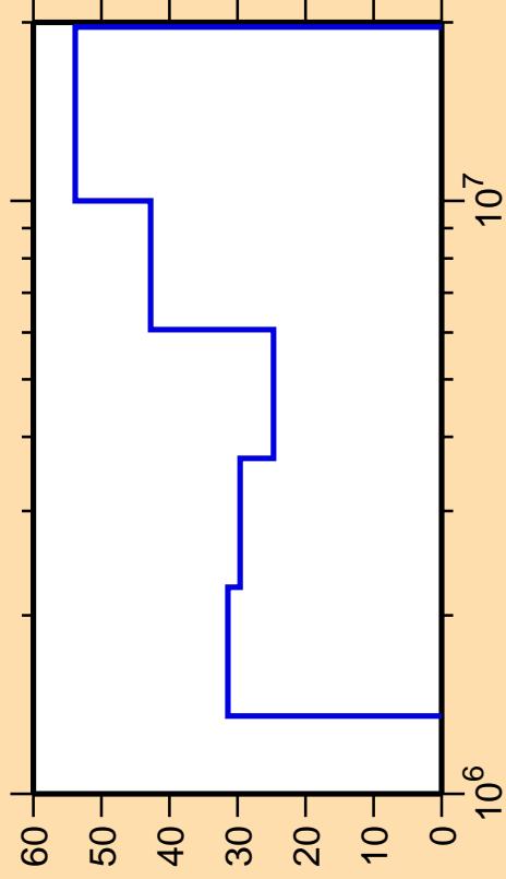
\Delta\sigma/\sigma vs. E for ^{72}\text{Zn}(n,n_4)
