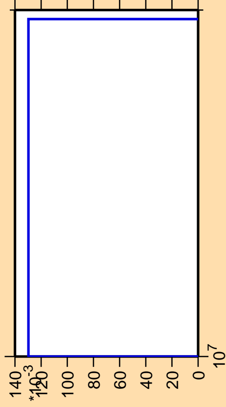
\Delta\sigma/\sigma vs. E for ^{72}\text{Zn}(n,nd)
