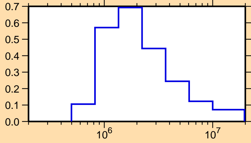
\sigma vs. E for ^{72}\text{Zn}(n,n_1)
