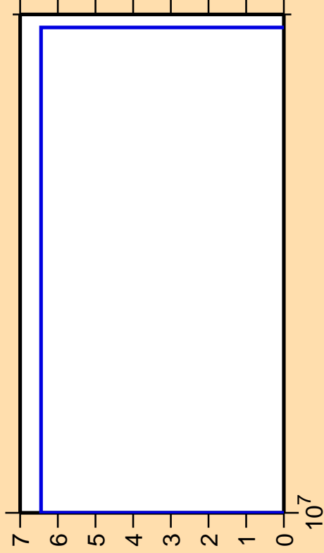
\Delta\sigma/\sigma vs. E for ^{72}\text{Zn}(n,nt)
