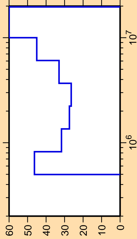
\Delta\sigma/\sigma vs. E for ^{72}\text{Zn}(n,n_1)
