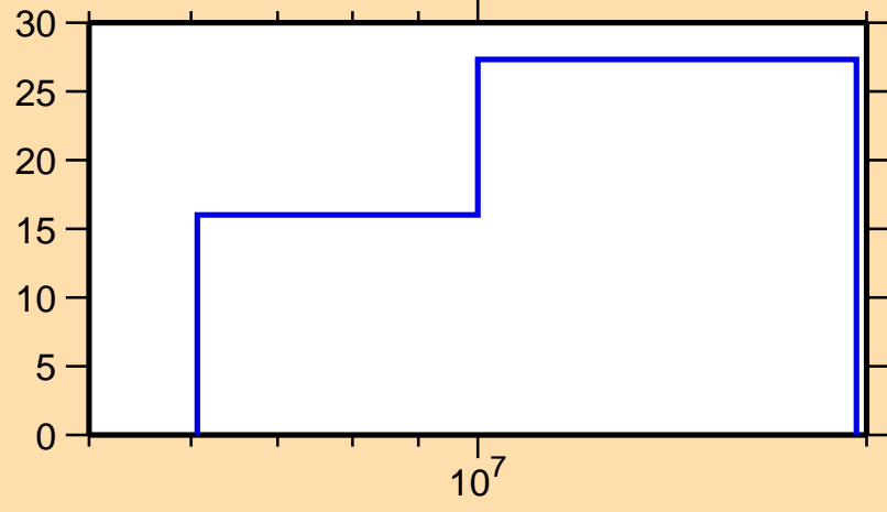
\Delta\sigma/\sigma vs. E for ^{72}\text{Zn}(n,el.)
