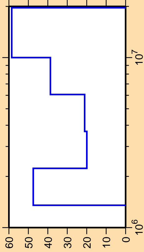
\Delta\sigma/\sigma vs. E for ^{72}\text{Zn}(n,n_2)
