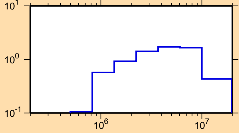
\sigma vs. E for ^{72}\text{Zn}(n,\text{inel.})
