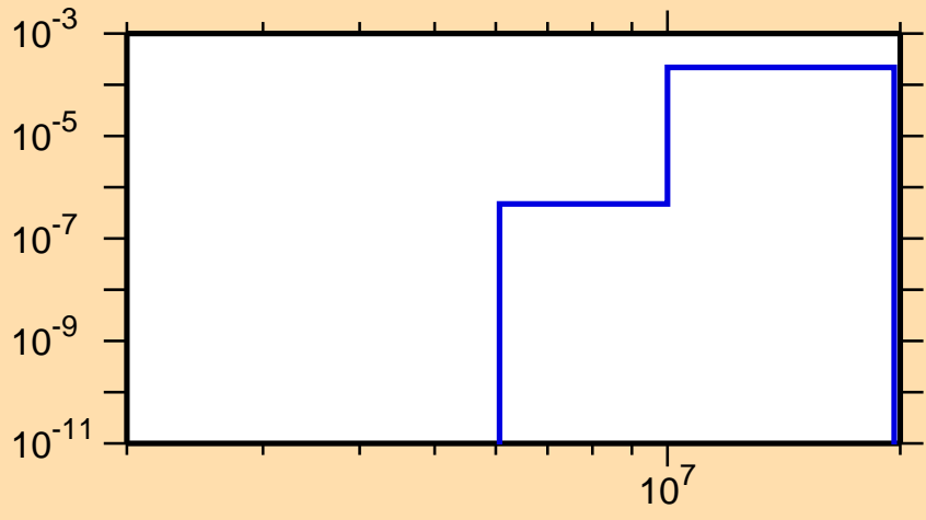
\sigma vs. E for ^{72}\text{Zn}(n,\alpha)
