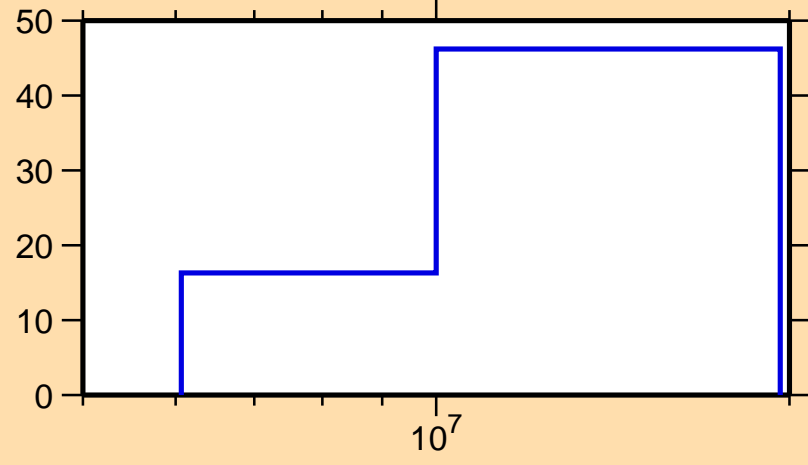
\Delta\sigma/\sigma vs. E for ^{72}\text{Zn}(n,ncont.)
