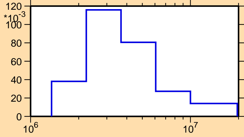
\sigma vs. E for ^{72}\text{Zn}(n,n_2)
