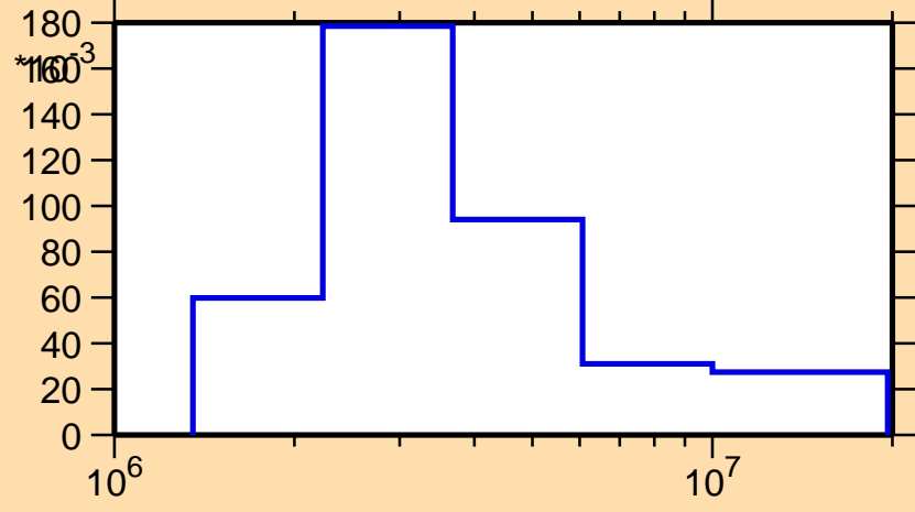
\sigma vs. E for ^{72}\text{Zn}(n,n_4)
