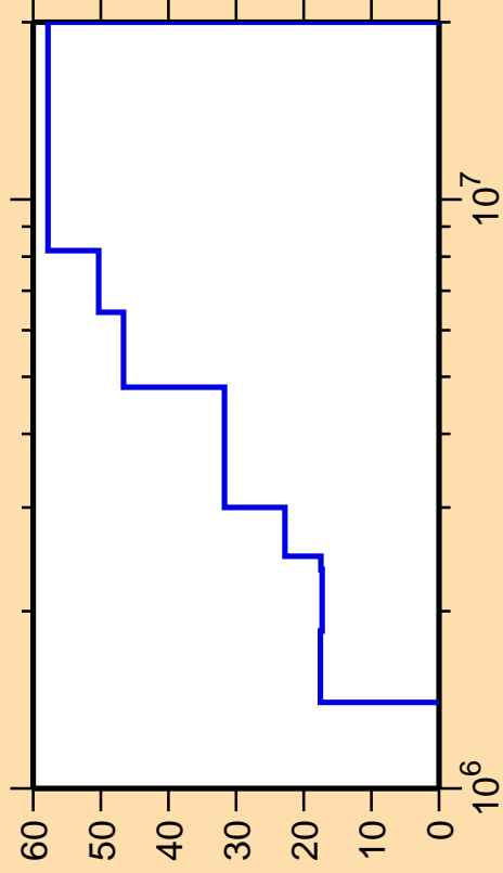
\Delta\sigma/\sigma vs. E for ^{72}\text{Zn}(n,n_3)
