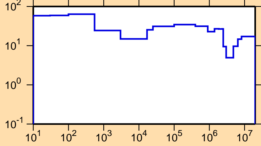
\Delta\sigma/\sigma vs. E for ^{72}\text{Zn}(n,\text{tot.})
