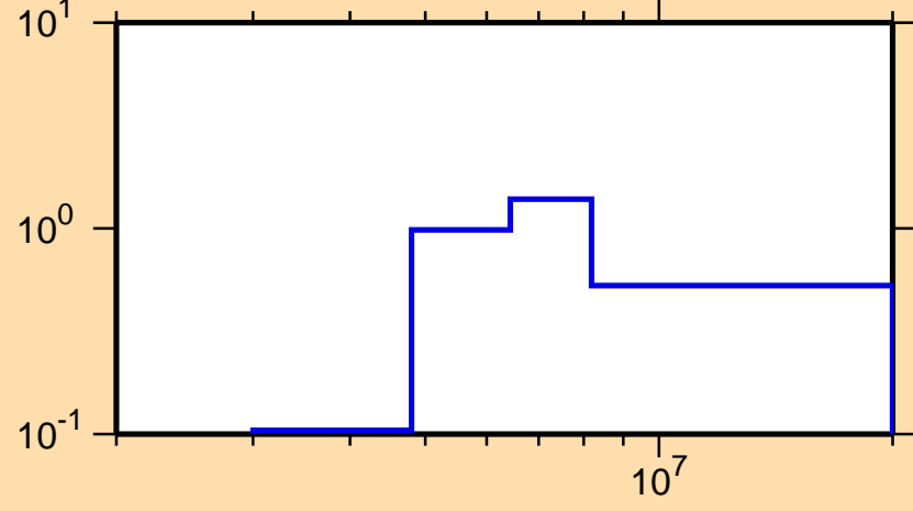
\sigma vs. E for ^{72}\text{Zn}(n,n\text{cont.})
