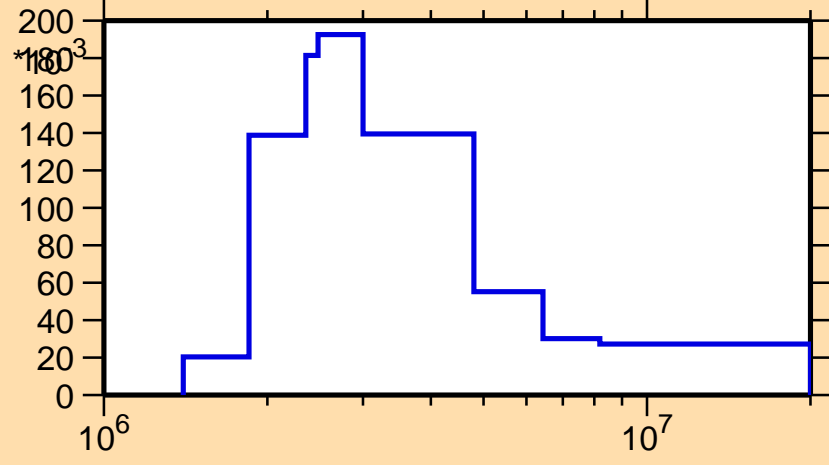
\sigma vs. E for ^{72}\text{Zn}(n,n_4)
