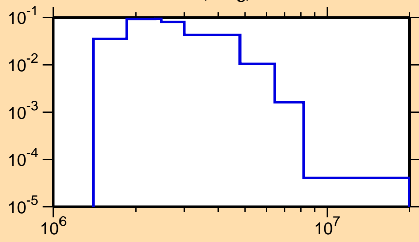
\sigma vs. E for ^{72}\text{Zn}(n,n_3)
