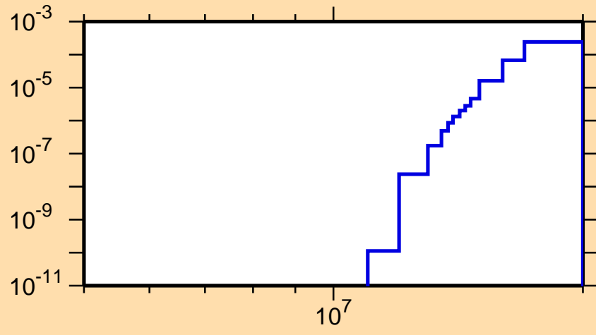
\sigma vs. E for ^{73}\text{Zn}(n,t)
