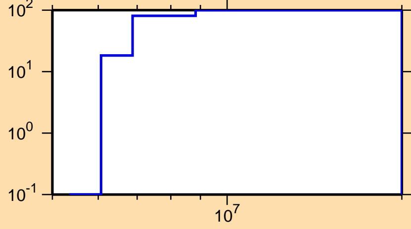
\Delta\sigma/\sigma vs. E for ^{73}\text{Zn}(n,p)
