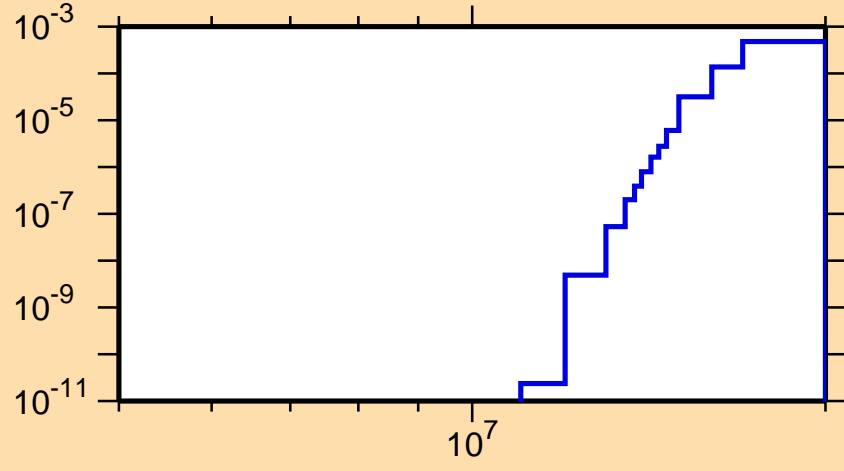
\sigma vs. E for ^{73}\text{Zn}(n,\alpha)
