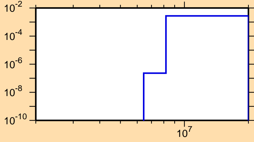
\sigma vs. E for ^{73}\text{Zn}(n,p)
