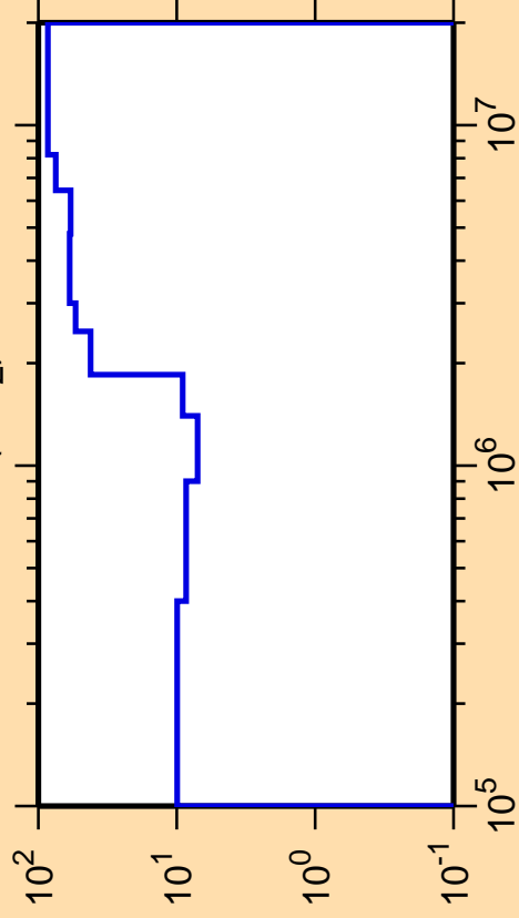
\Delta\sigma/\sigma vs. E for ^{73}\text{Zn}(n,n_2)
