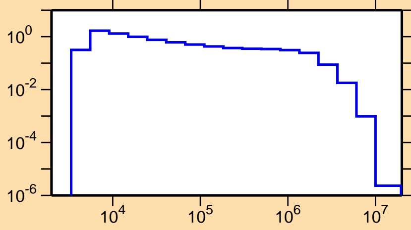
\sigma vs. E for ^{73}\text{Zn}(n,n_2)
