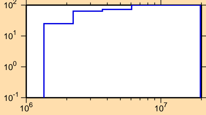
\Delta\sigma/\sigma vs. E for ^{73}\text{Zn}(n,n_1)
