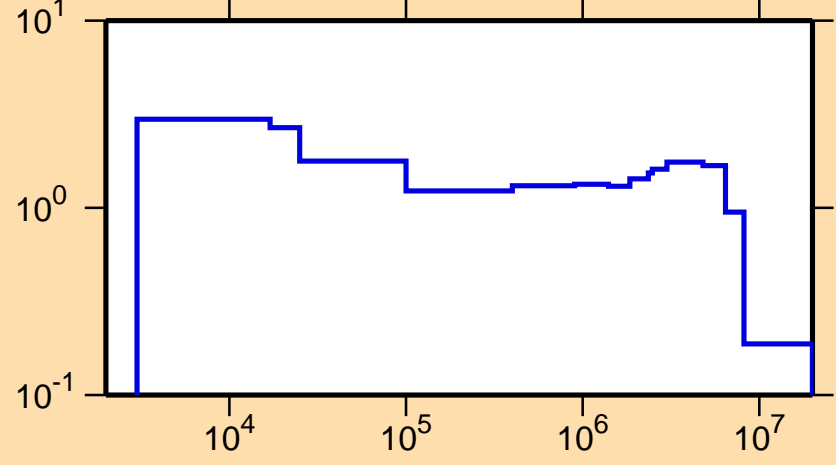
\sigma vs. E for ^{73}\text{Zn}(n,\text{inel.})
