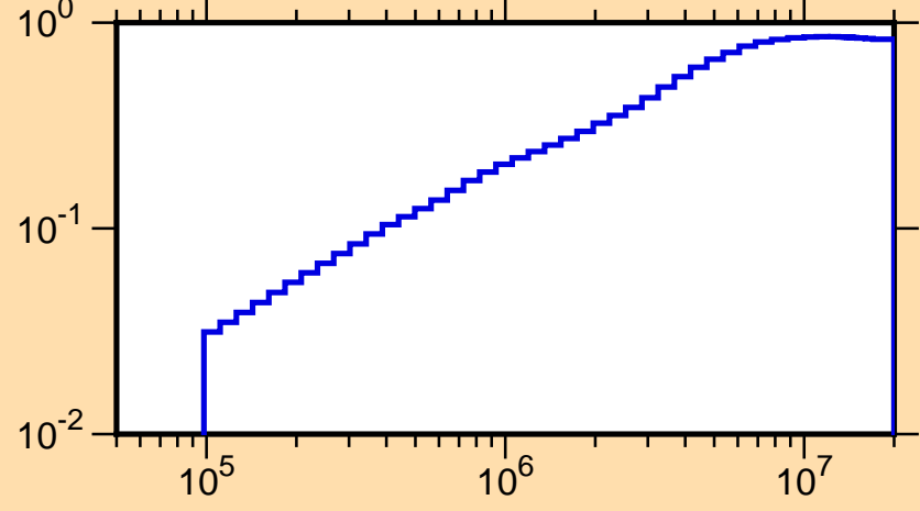
\mu vs. E for ^{74}\text{Zn}(\text{mt251})
