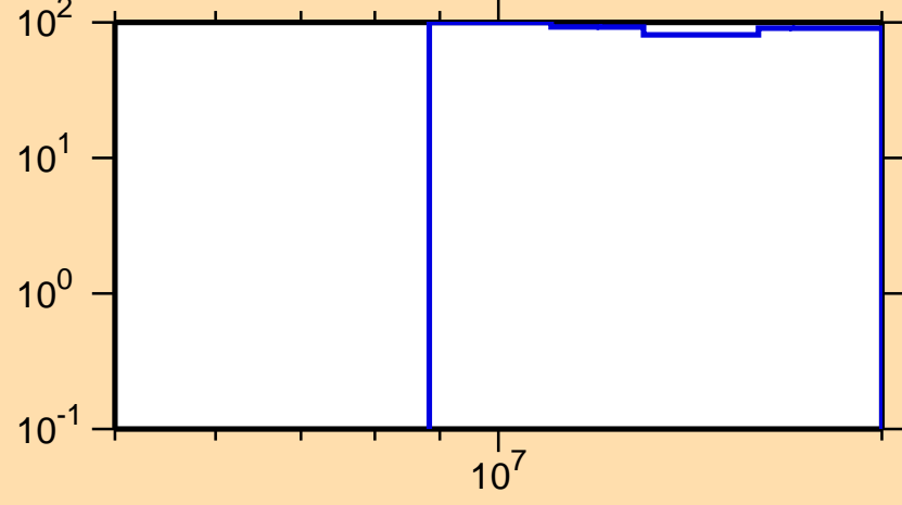
\Delta\sigma/\sigma vs. E for ^{74}\text{Zn}(n,p)
