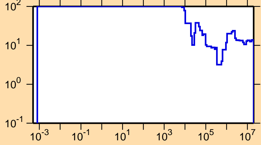
\Delta\sigma/\sigma vs. E for ^{74}\text{Zn}(n,\text{tot.})
