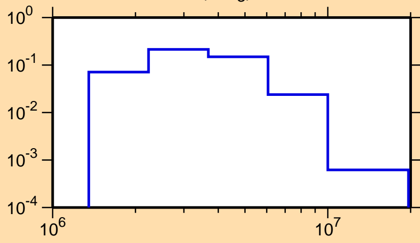
\sigma vs. E for ^{74}\text{Zn}(n,n_3)
