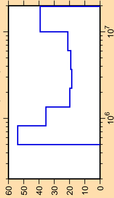
\Delta\sigma/\sigma vs. E for ^{74}\text{Zn}(n,\text{inel.})
