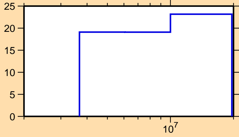
\Delta\sigma/\sigma vs. E for ^{74}\text{Zn}(n,n\text{onel.})
