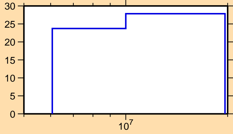
\Delta\sigma/\sigma vs. E for ^{74}\text{Zn}(n,el.)
