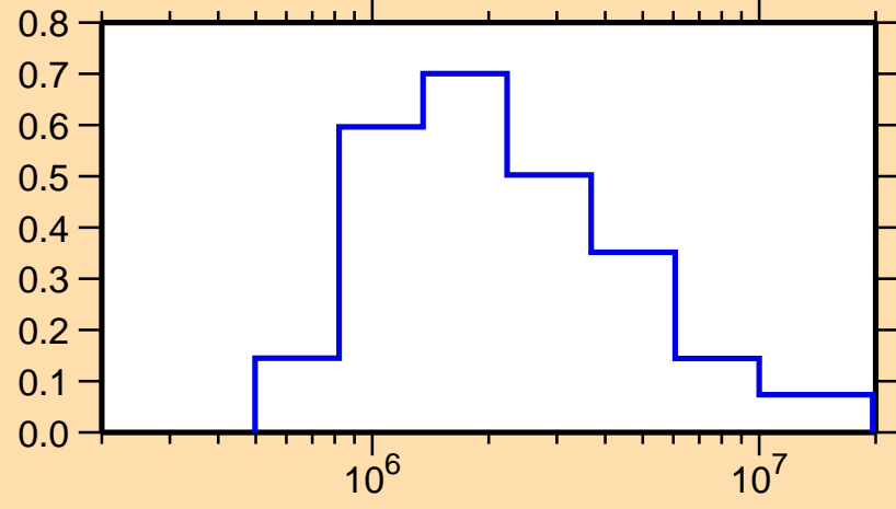
\sigma vs. E for ^{74}\text{Zn}(n,n_1)
