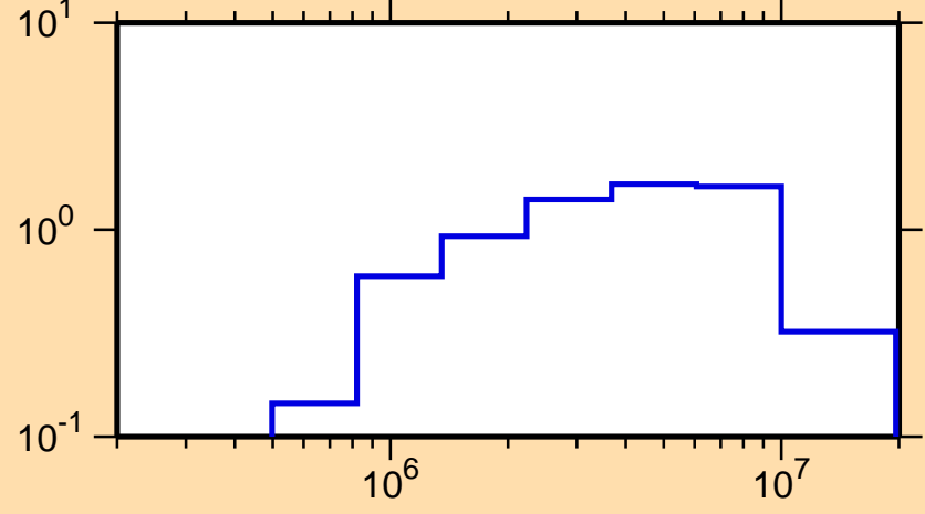
\sigma vs. E for ^{74}\text{Zn}(n,\text{inel.})
