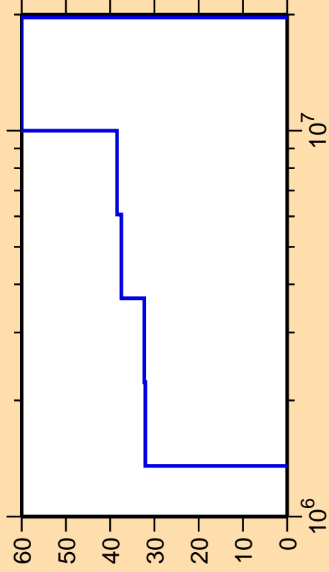
\Delta\sigma/\sigma vs. E for ^{74}\text{Zn}(n,n_3)
