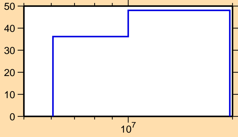
\Delta\sigma/\sigma vs. E for ^{74}\text{Zn}(n,ncont.)
