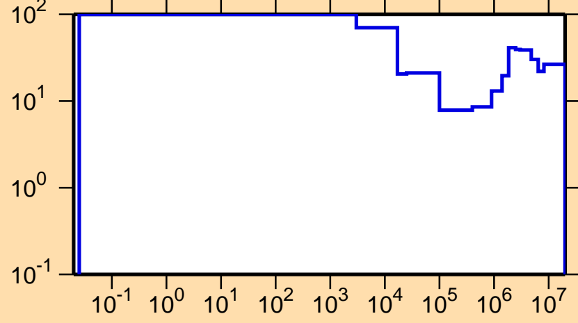
\Delta\sigma/\sigma vs. E for ^{74}\text{Zn}(n,\text{el.})
