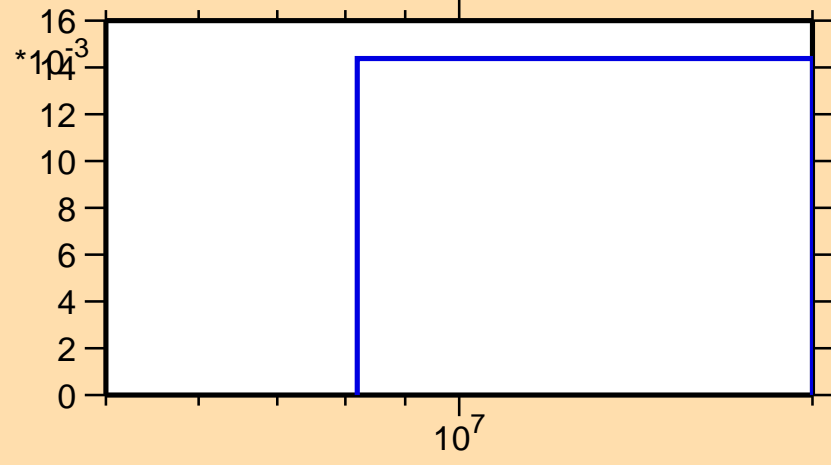
\sigma vs. E for ^{74}\text{Zn}(n,3n)
