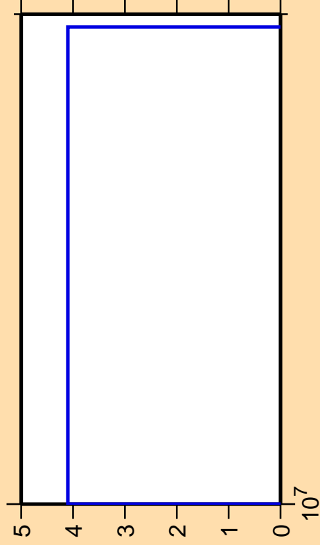
\Delta\sigma/\sigma vs. E for ^{75}\text{Zn}(n,2n\alpha)
