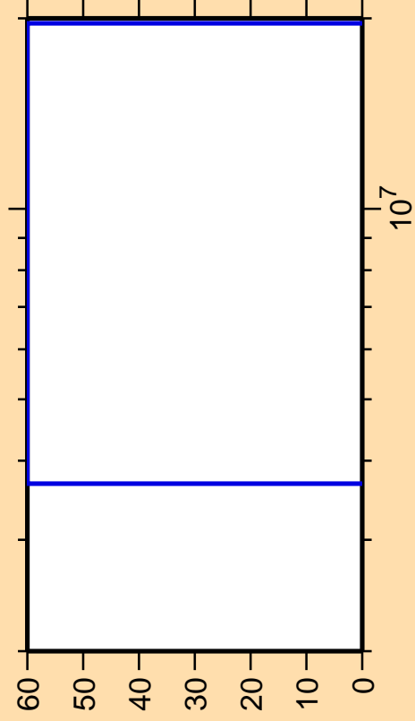
\Delta\sigma/\sigma vs. E for ^{75}\text{Zn}(n,n_1)
