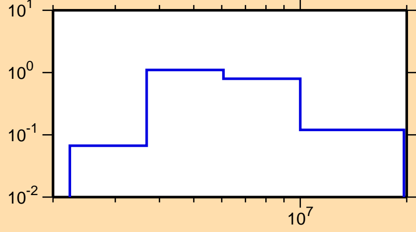
\sigma vs. E for ^{75}\text{Zn}(n,n\text{cont.})
