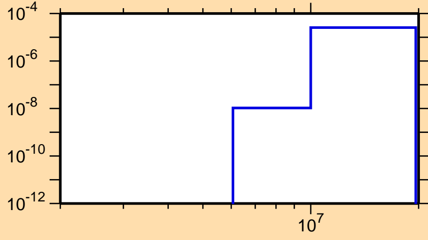
\sigma vs. E for ^{75}\text{Zn}(n,\alpha)
