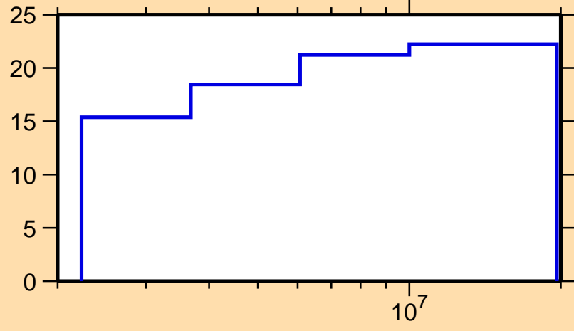
\Delta\sigma/\sigma vs. E for ^{75}\text{Zn}(n,n\text{onel.})
