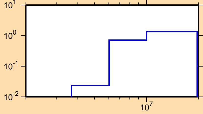
\sigma vs. E for ^{75}\text{Zn}(n,2n)
