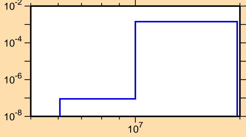
\sigma vs. E for ^{75}\text{Zn}(n,p)
