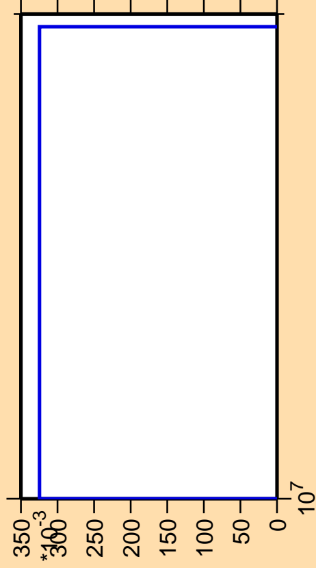
\Delta\sigma/\sigma vs. E for ^{75}\text{Zn}(n,nt)
