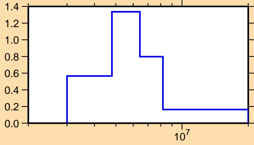
\sigma vs. E for ^{75}\text{Zn}(n,n\text{cont.})
