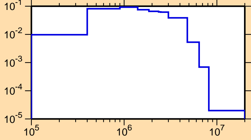
\sigma vs. E for ^{75}\text{Zn}(n,n_3)
