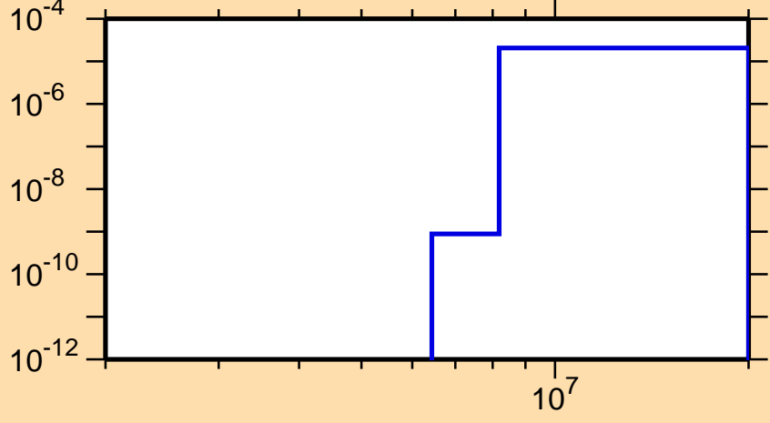
\sigma vs. E for ^{75}\text{Zn}(n,\alpha)
