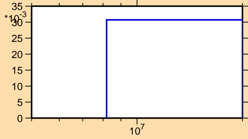
\sigma vs. E for ^{75}\text{Zn}(n,3n)
