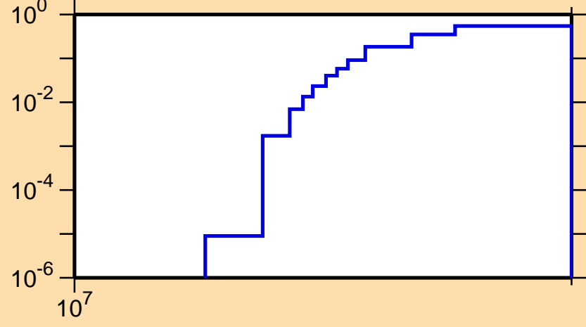
\sigma vs. E for ^{76}\text{Zn}(n,3n)
