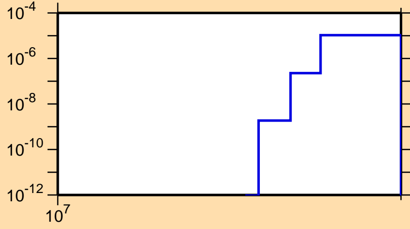
\sigma vs. E for ^{76}\text{Zn}(n,t)
