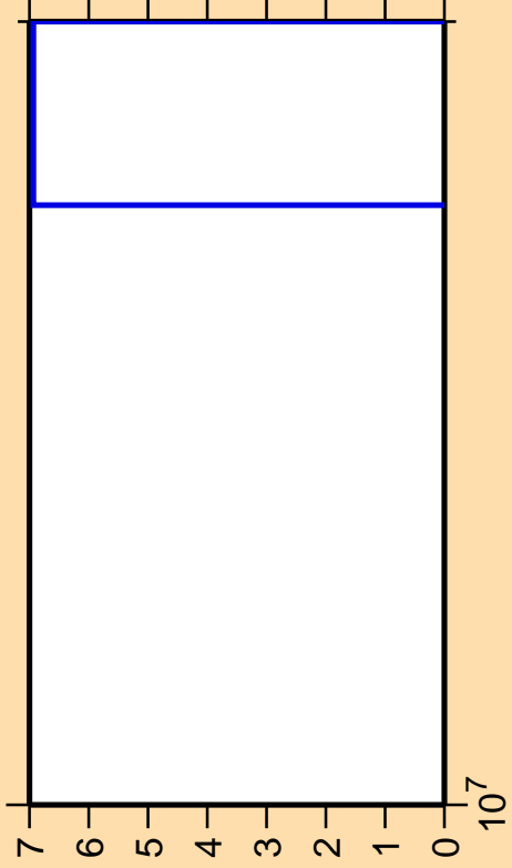
\Delta\sigma/\sigma vs. E for ^{76}\text{Zn}(n,nt)
