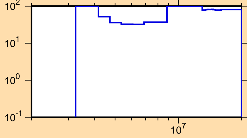
\Delta\sigma/\sigma vs. E for ^{76}\text{Zn}(n,n\text{cont.})
