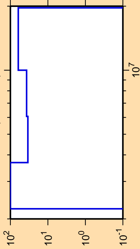
\Delta\sigma/\sigma vs. E for ^{76}\text{Zn}(n,ncont.)
