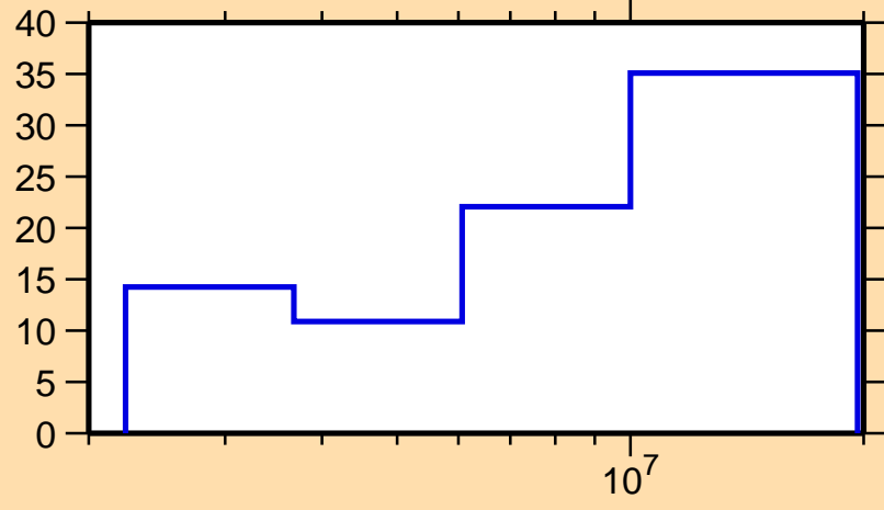
\Delta\sigma/\sigma vs. E for ^{76}\text{Zn}(n,inel.)
