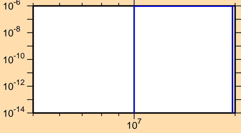
\sigma vs. E for ^{76}\text{Zn}(n,\alpha)
