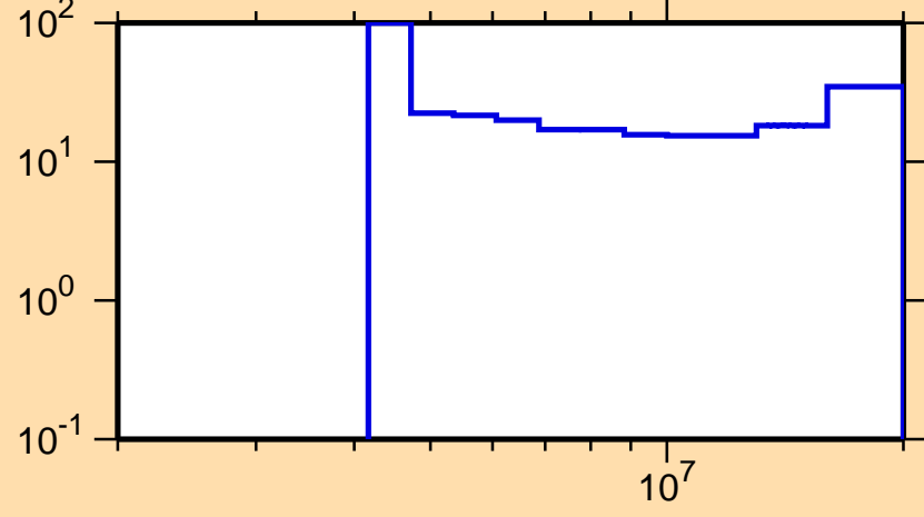
\Delta\sigma/\sigma vs. E for ^{77}\text{Zn}(n,2n)
