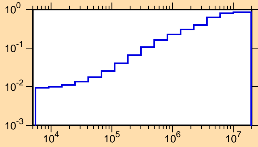
\mu vs. E for ^{77}\text{Zn(mt251)}
