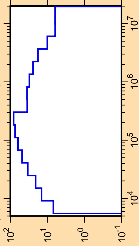
\Delta\mu/\mu vs. E for ^{77}\text{Zn(mt251)}
