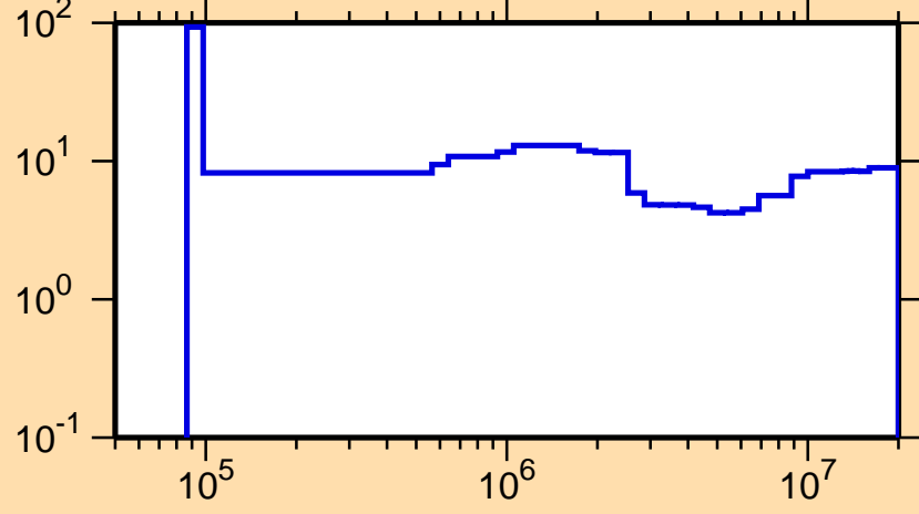
\Delta\sigma/\sigma vs. E for ^{77}\text{Zn}(n,\text{tot.})
