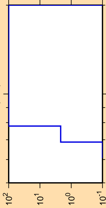
\Delta\sigma/\sigma vs. E for ^{77}\text{Zn}(n,\alpha)
