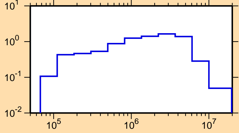
\sigma vs. E for ^{77}\text{Zn}(n,\text{inel.})
