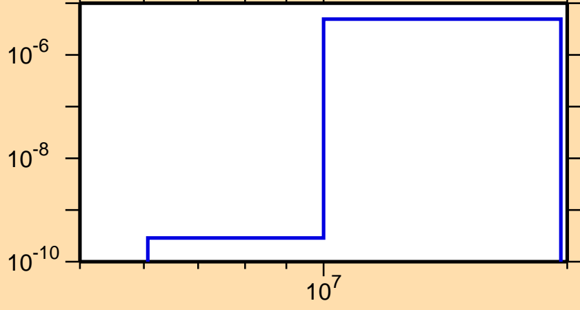
\sigma vs. E for ^{77}\text{Zn}(n,\alpha)
