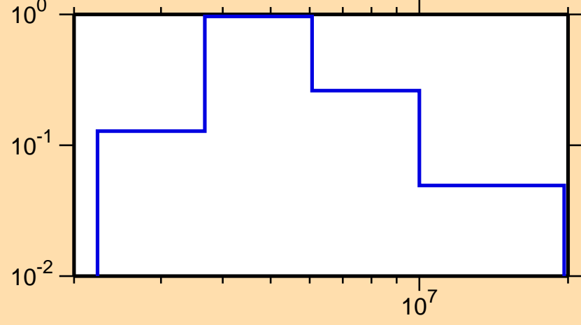
\sigma vs. E for ^{77}\text{Zn}(n,n\text{cont.})
