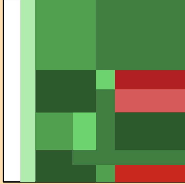
\Delta\sigma/\sigma vs. E for ^{77}\text{Zn}(n,n\text{cont.})
