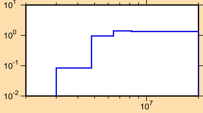
\sigma vs. E for ^{77}\text{Zn}(n,2n)
