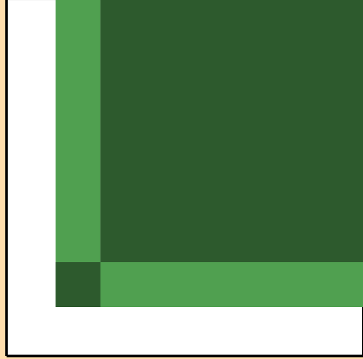
\sigma vs. E for ^{78}\text{Zn}(n,3n)
