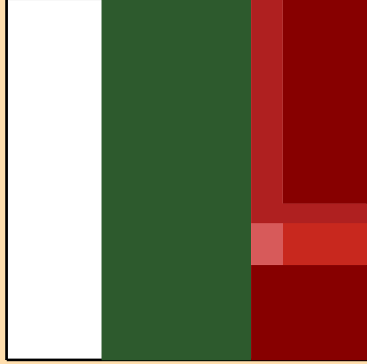
\Delta\sigma/\sigma vs. E for ^{78}\text{Zn}(n,p)
