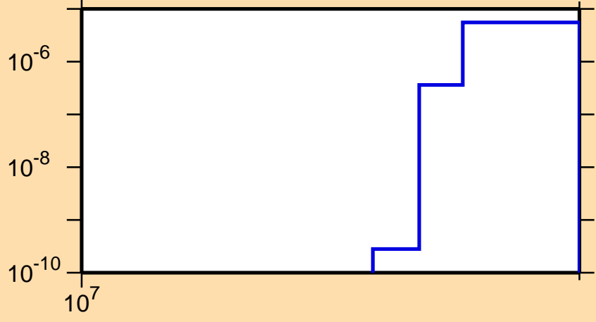
\sigma vs. E for ^{80}\text{Zr}(n,2n)
