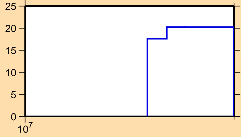
\Delta\sigma/\sigma vs. E for ^{80}\text{Zr}(n,\text{nonel.})
