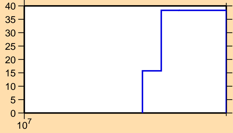
\Delta\sigma/\sigma vs. E for ^{80}\text{Zr}(n,\text{el.})
