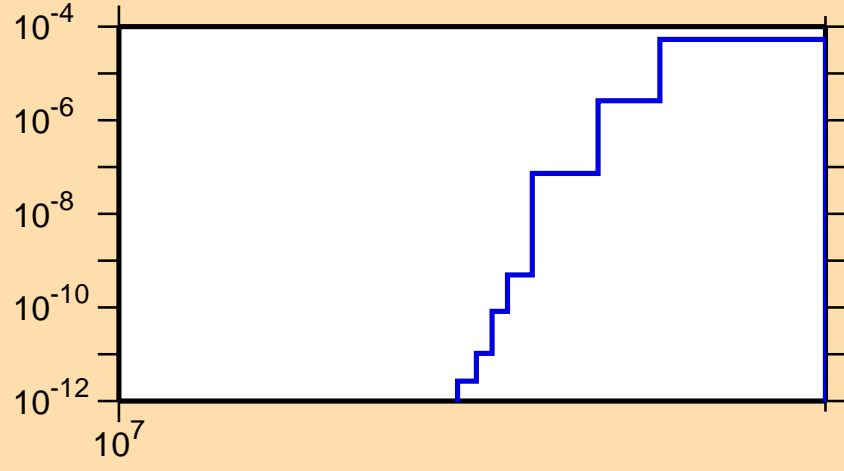
\sigma vs. E for ^{80}\text{Zr}(n,\text{pt})
