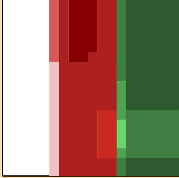
\Delta\sigma/\sigma vs. E for ^{80}\text{Zr}(n,n\text{cont.})
