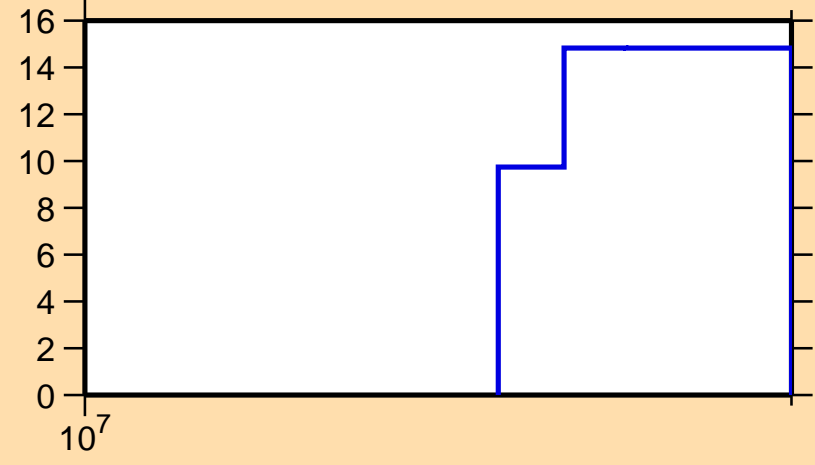
\Delta\sigma/\sigma vs. E for ^{80}\text{Zr}(n,\text{tot.})
