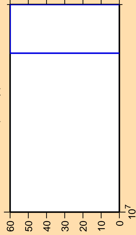
\Delta\sigma/\sigma vs. E for ^{80}\text{Zr}(n,2np)
