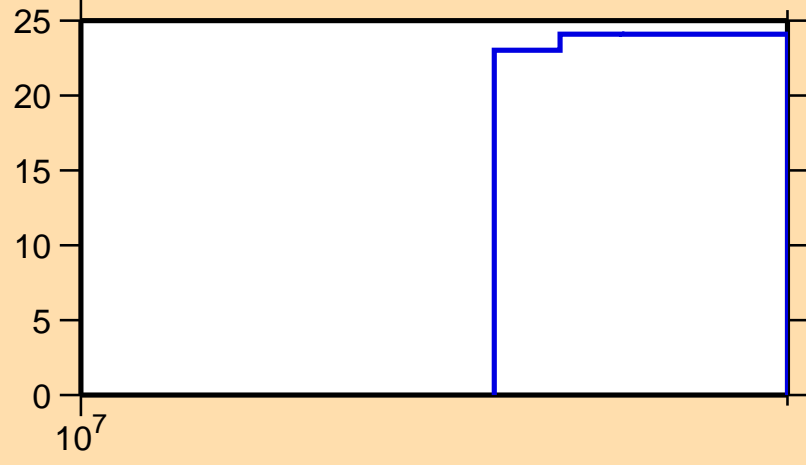
\Delta\sigma/\sigma vs. E for ^{80}\text{Zr}(n,\text{inel.})
