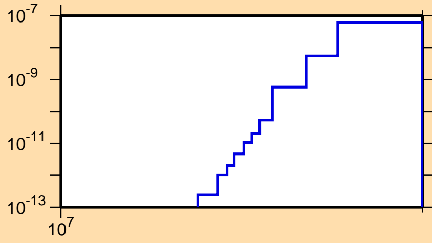
\sigma vs. E for ^{80}\text{Zr}(\text{mt117})
