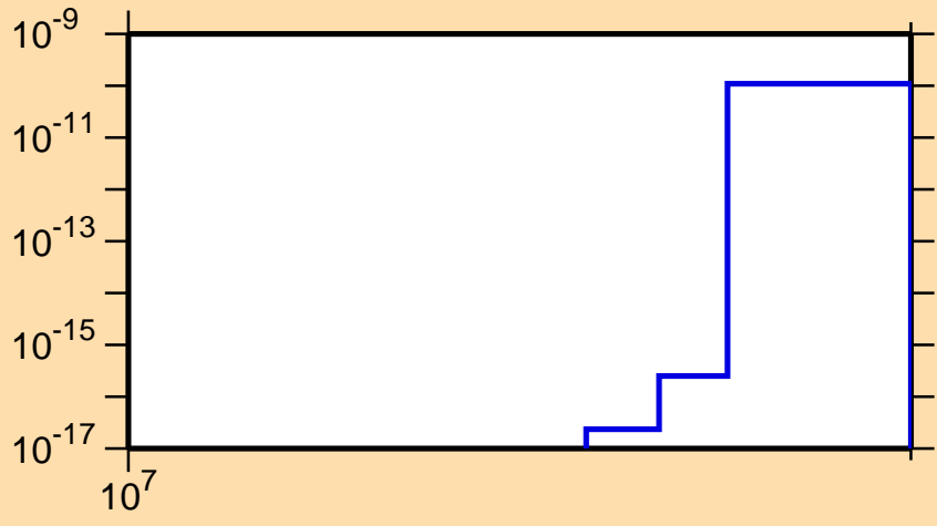
\sigma vs. E for ^{80}\text{Zr}(n,\text{nd})
