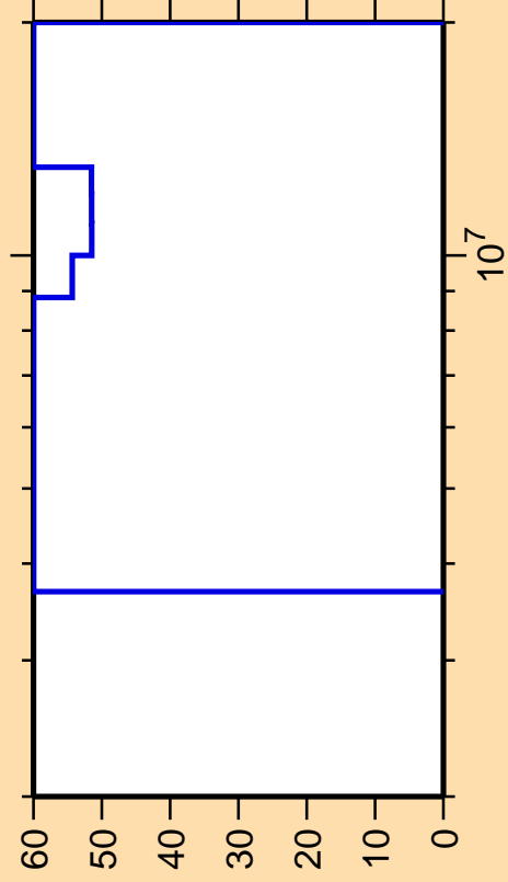
\Delta\sigma/\sigma vs. E for ^{80}\text{Zr}(n,\gamma)
