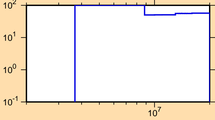
\Delta\sigma/\sigma vs. E for ^{80}\text{Zr}(n,n\text{cont.})
