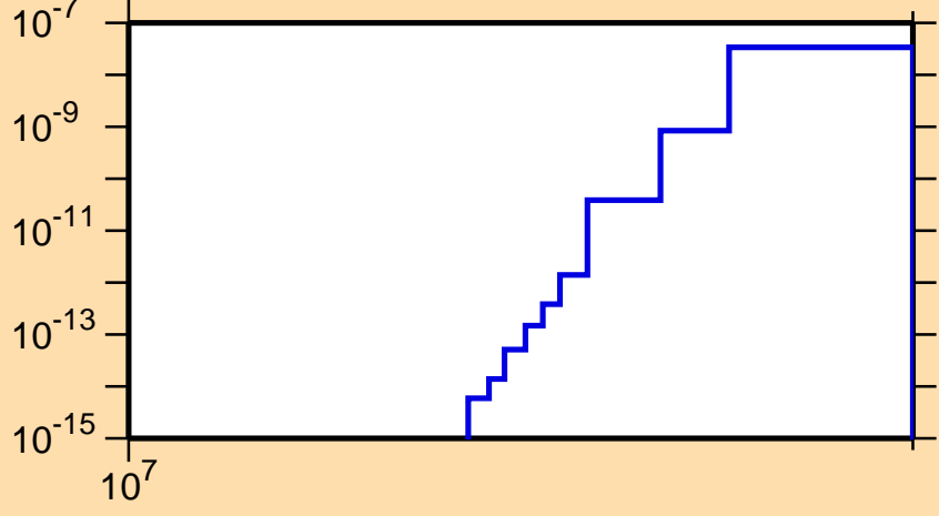
\sigma vs. E for ^{80}\text{Zr} (mt 45)
