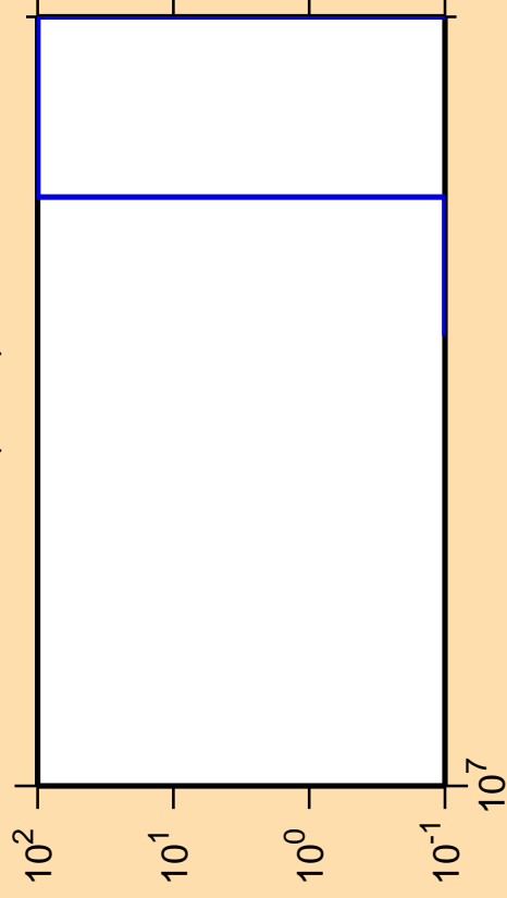
\Delta\sigma/\sigma vs. E for ^{80}\text{Zr}(n,\text{nd})
