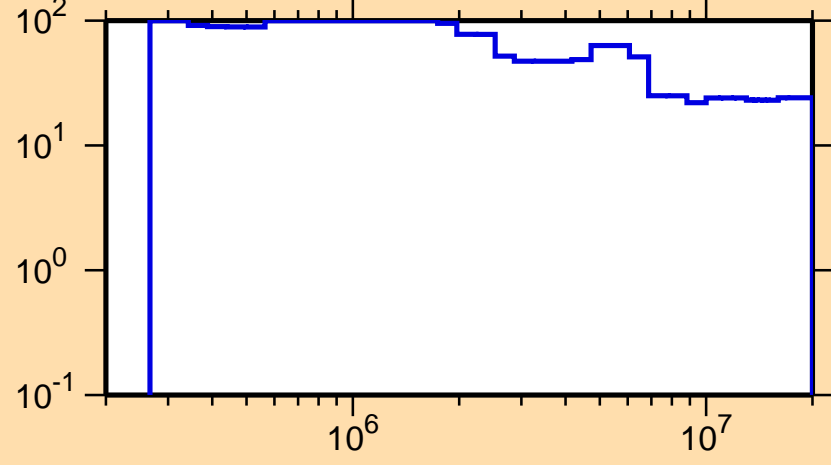
\Delta\sigma/\sigma vs. E for ^{80}\text{Zr}(n,\text{inel.})
