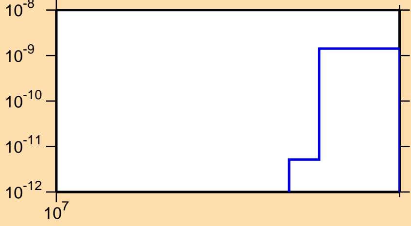
\sigma vs. E for ^{80}\text{Zr} (mt 34)
