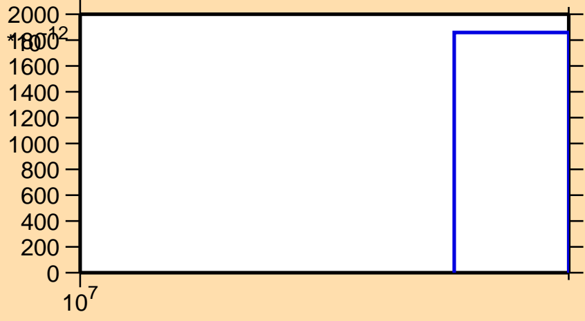
\sigma vs. E for ^{80}\text{Zr}(n,2np)
