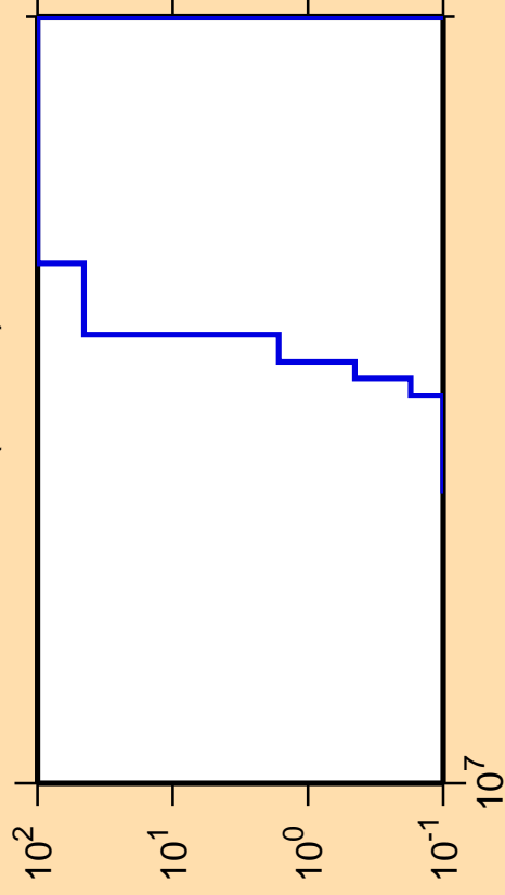
\Delta\sigma/\sigma vs. E for ^{80}\text{Zr} (mt 45)
