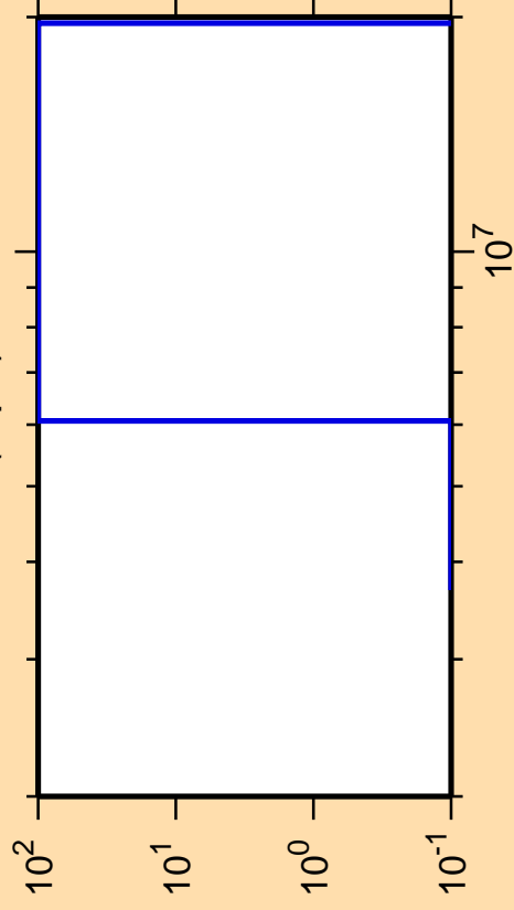
\Delta\sigma/\sigma vs. E for ^{80}\text{Zr}(n,pd)
