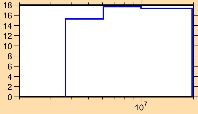
\Delta\sigma/\sigma vs. E for ^{80}\text{Zr}(n,nonel.)
