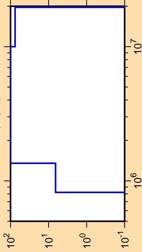
\Delta\sigma/\sigma vs. E for ^{80}\text{Zr}(n,p\alpha)
