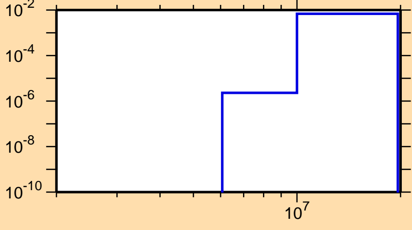
\sigma vs. E for ^{80}\text{Zr}(n,pd)
