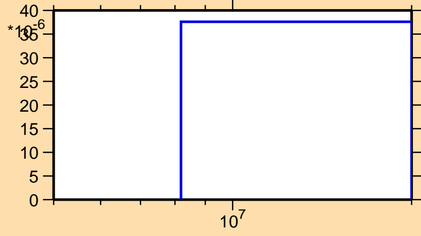
\sigma vs. E for ^{80}\text{Zr}(n,t)
