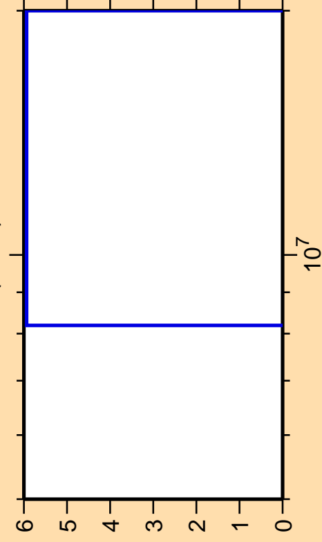
\Delta\sigma/\sigma vs. E for ^{80}\text{Zr}(n,\text{nd})
