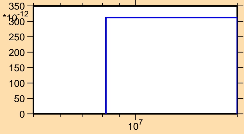
\sigma vs. E for ^{80}\text{Zr}(\text{mt } 45)
