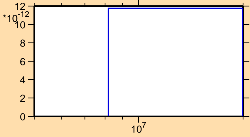
\sigma vs. E for ^{80}\text{Zr}(\text{mt } 34)
