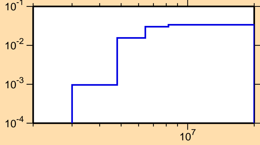
\sigma vs. E for ^{80}\text{Zr}(n,n\text{cont.})
