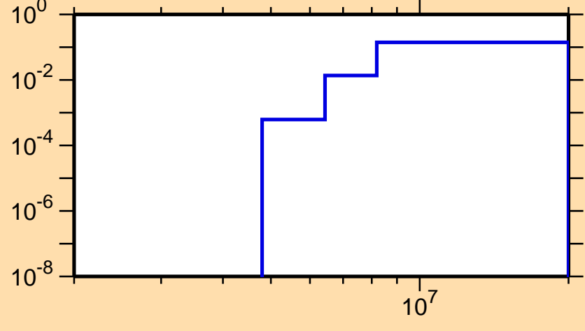
\sigma vs. E for ^{80}\text{Zr}(n,np)
