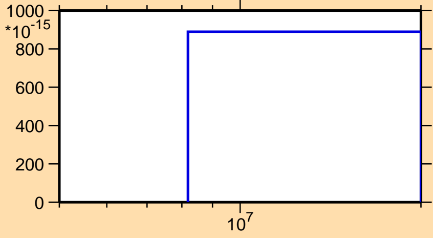
\sigma vs. E for ^{80}\text{Zr}(n,\text{nd})
