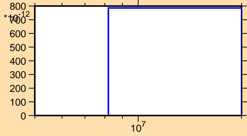
\sigma vs. E for ^{80}\text{Zr}(\text{mt117})
