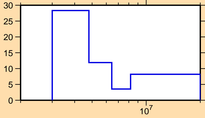
\Delta\sigma/\sigma vs. E for ^{80}\text{Zr}(n,tot.)
