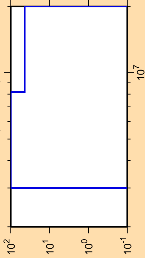
\Delta\sigma/\sigma vs. E for ^{80}\text{Zr}(n,ncont.)
