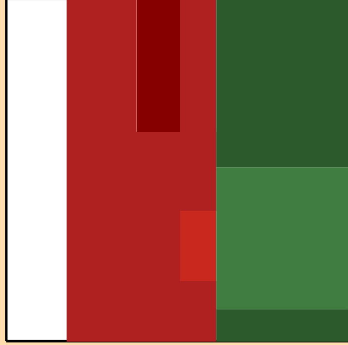
\Delta\sigma/\sigma vs. E for ^{80}\text{Zr}(n,ncont.)
