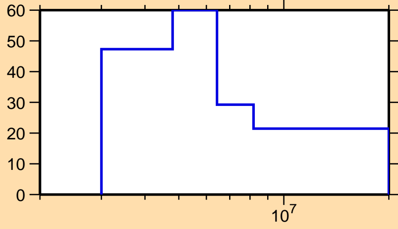
\Delta\sigma/\sigma vs. E for ^{80}\text{Zr}(n,inel.)
