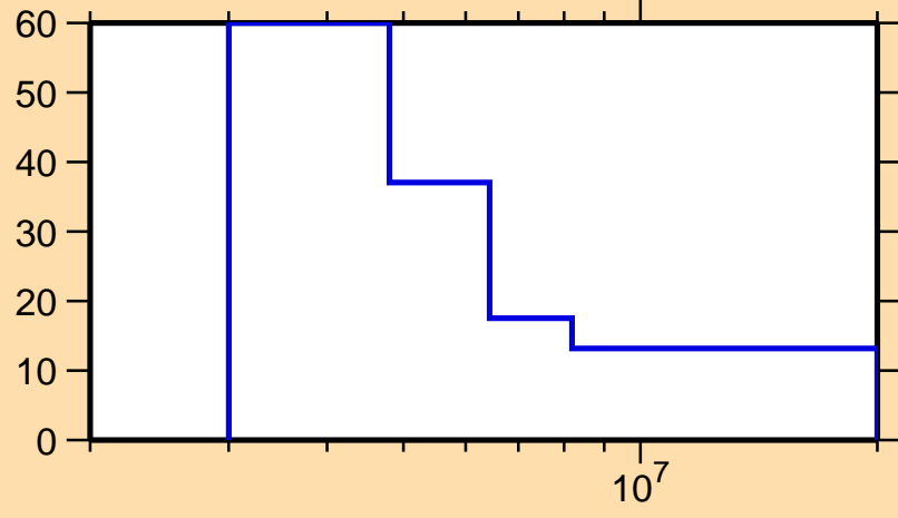
\Delta\sigma/\sigma vs. E for ^{80}\text{Zr}(n,el.)
