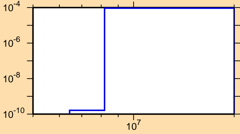
\sigma vs. E for ^{80}\text{Zr}(n,\alpha)
