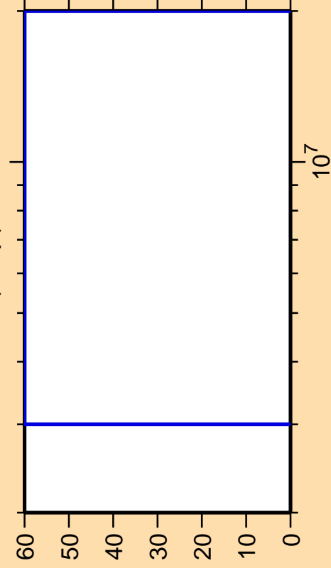
\Delta\sigma/\sigma vs. E for ^{80}\text{Zr}(n,np)
