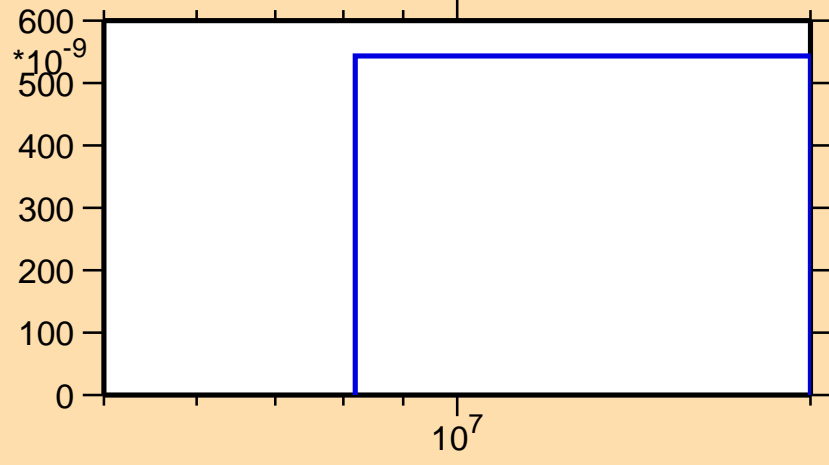
\sigma vs. E for ^{80}\text{Zr}(n,\text{pt})
