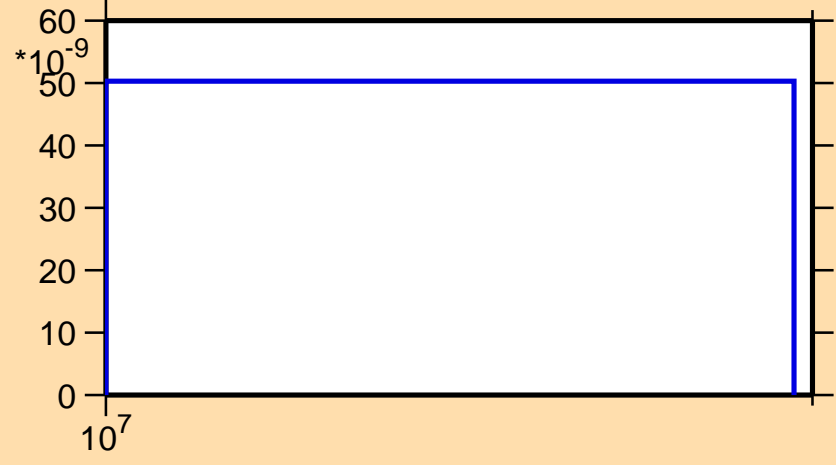
\sigma vs. E for ^{81}\text{Zr}(n,2np)
