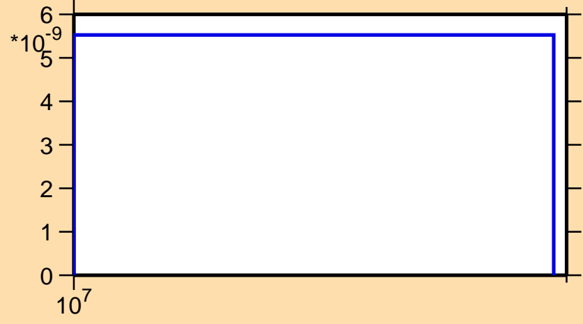
\sigma vs. E for ^{81}\text{Zr}(\text{mt } 34)
