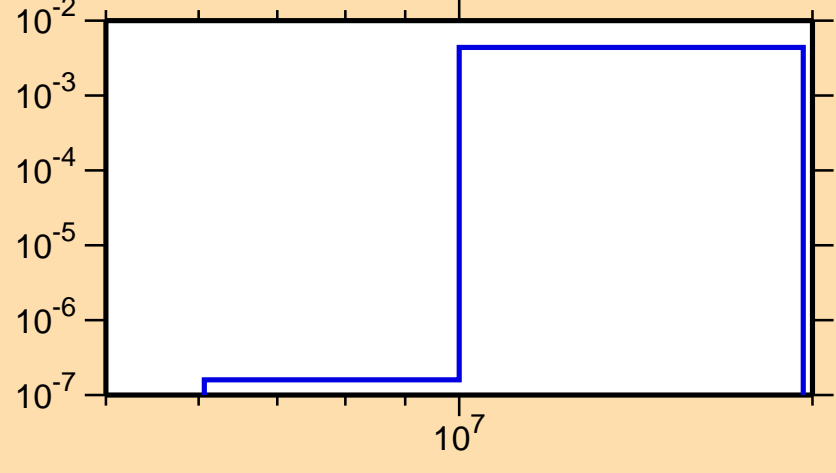
\sigma vs. E for ^{81}\text{Zr}(n,pd)
