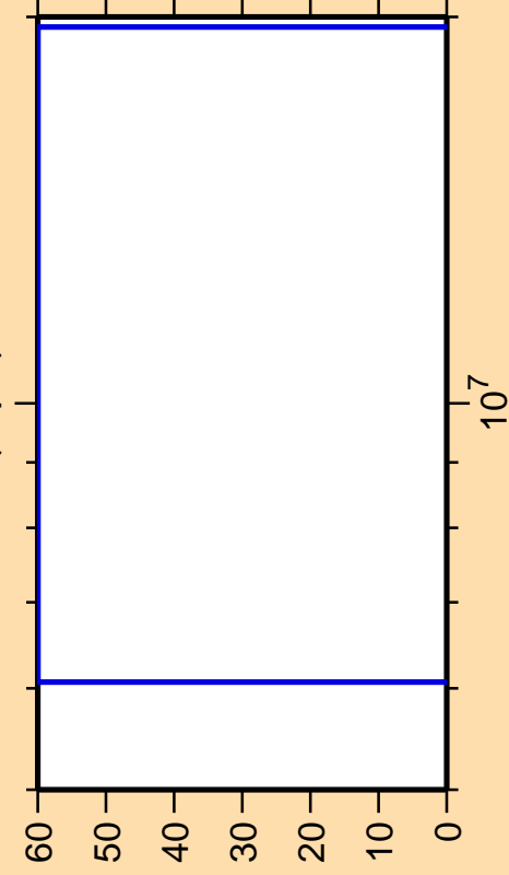
\Delta\sigma/\sigma vs. E for ^{81}\text{Zr}(n,pd)
