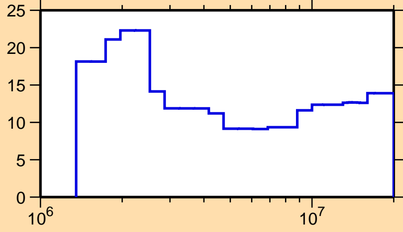
\Delta\sigma/\sigma vs. E for ^{82}\text{Zr}(n,nonel.)
