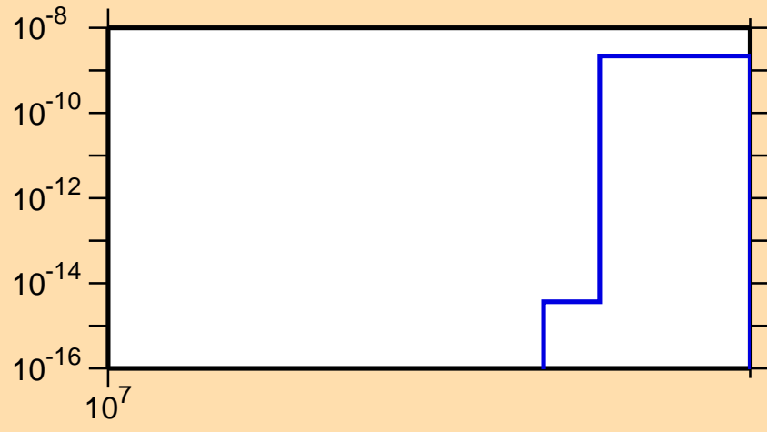
\sigma vs. E for ^{82}\text{Zr}(n,\text{nd})
