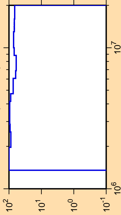
\Delta\sigma/\sigma vs. E for ^{82}\text{Zr}(n,ncont.)
