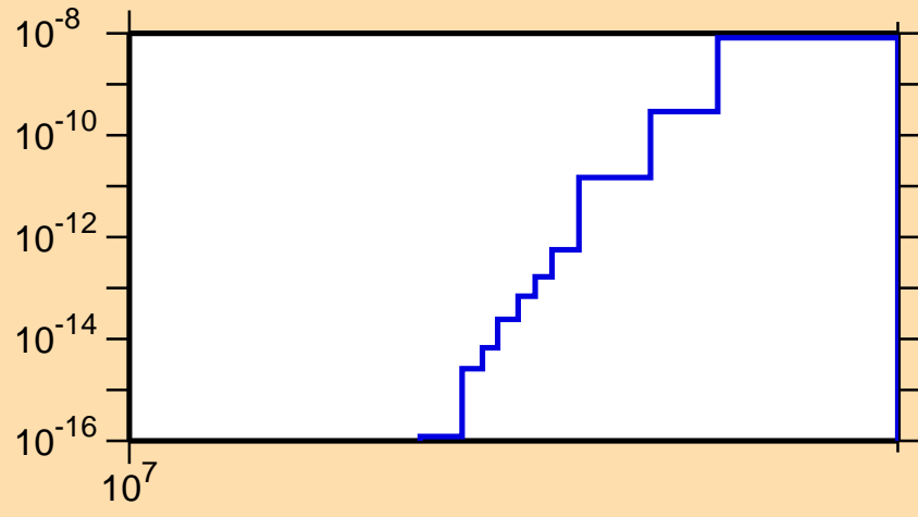
\sigma vs. E for ^{82}\text{Zr}(\text{mt117})
