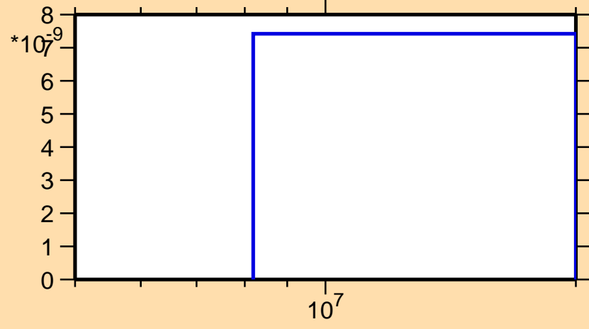
\sigma vs. E for ^{82}\text{Zr}(n,pt)
