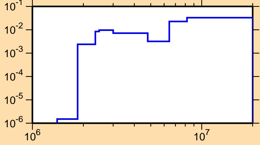
\sigma vs. E for ^{82}\text{Zr}(n,n\text{cont.})
