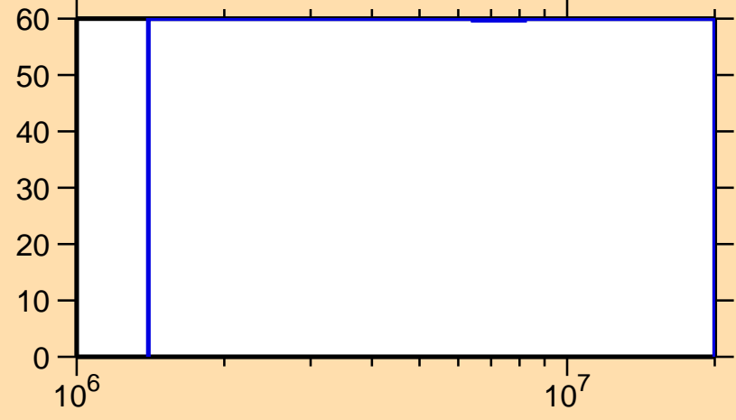
\Delta\sigma/\sigma vs. E for ^{82}\text{Zr}(n,ncont.)
