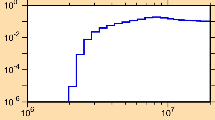
\sigma vs. E for ^{83}\text{Zr}(n,n\text{cont.})
