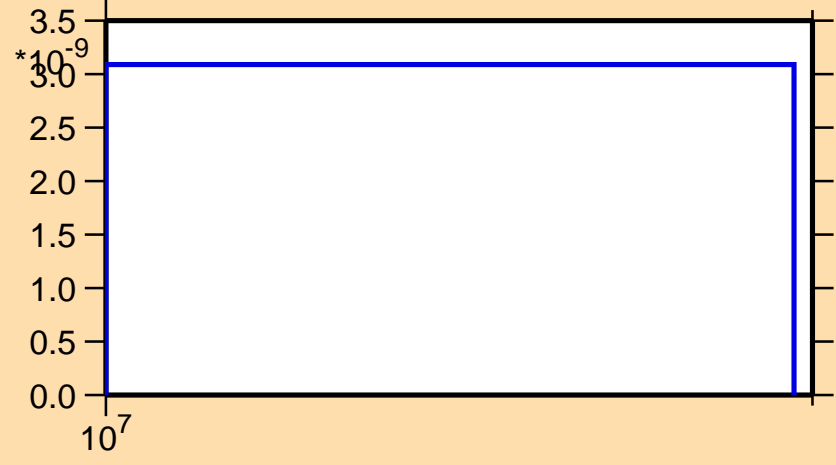
\sigma vs. E for ^{83}\text{Zr}(\text{mt } 45)
