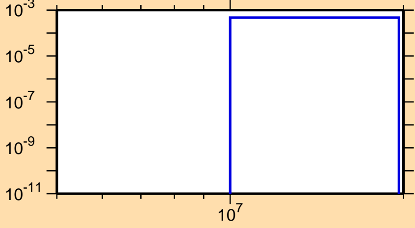
\sigma vs. E for ^{83}\text{Zr}(n,pd)
