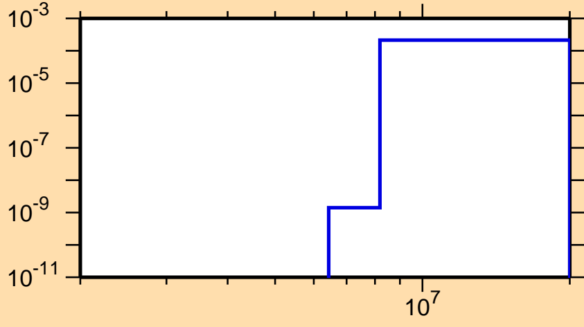
\sigma vs. E for ^{83}\text{Zr}(n,\text{He}3)
