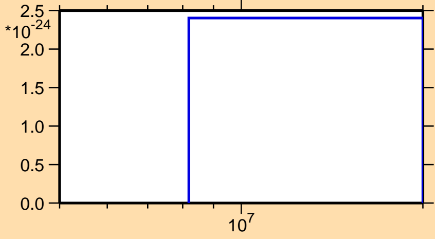
\sigma vs. E for ^{83}\text{Zr}(n,nt)
