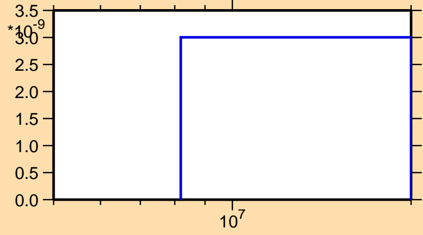
\sigma vs. E for ^{83}\text{Zr} (mt 45)
