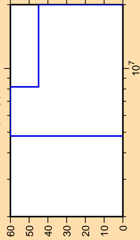
\Delta\sigma/\sigma vs. E for ^{83}\text{Zr}(n,np)
