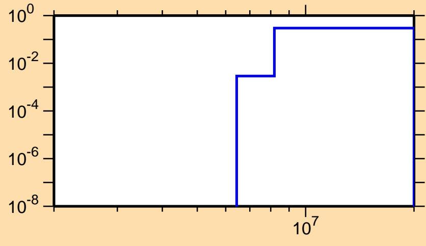
\sigma vs. E for ^{83}\text{Zr}(n,np)
