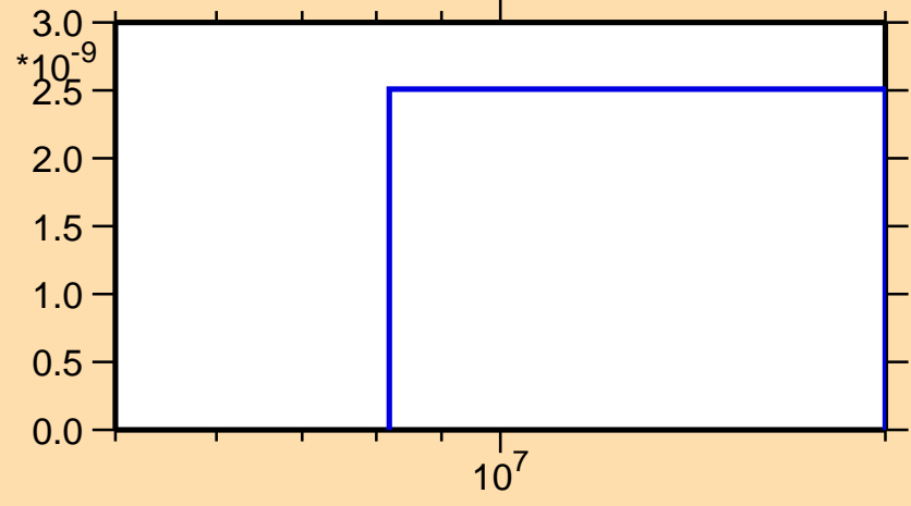
\sigma vs. E for ^{83}\text{Zr}(\text{mt } 34)
