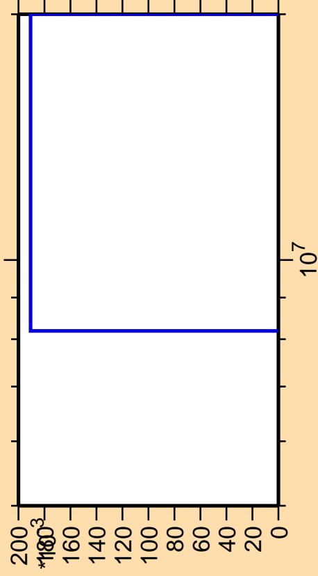
\Delta\sigma/\sigma vs. E for ^{83}\text{Zr}(n,2n\alpha)
