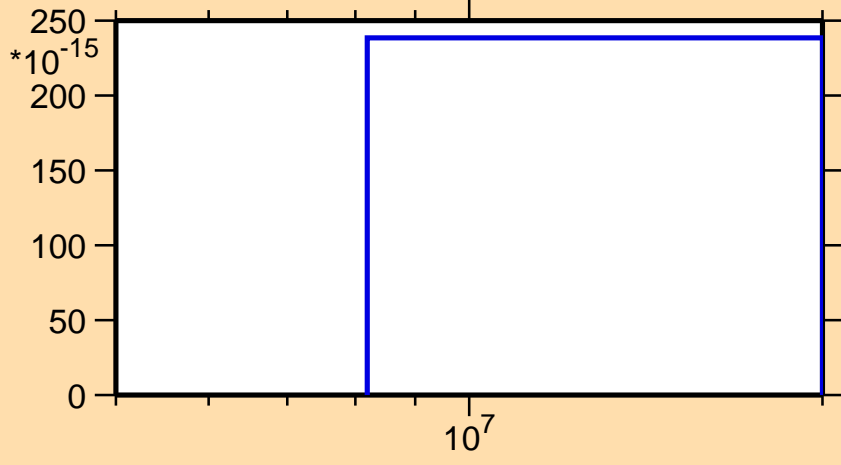
\sigma vs. E for ^{83}\text{Zr}(n,2n\alpha)
