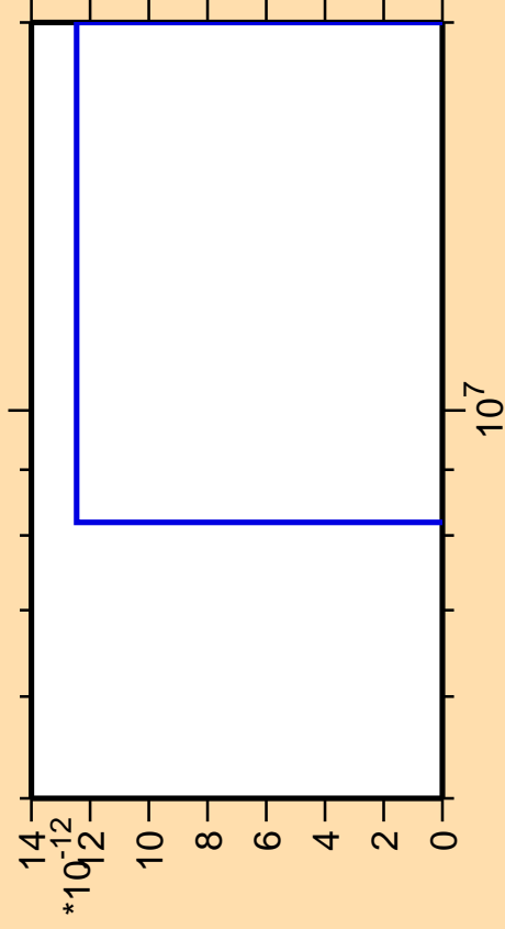
\Delta\sigma/\sigma vs. E for ^{83}\text{Zr}(n,nt)
