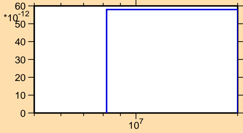
\sigma vs. E for ^{83}\text{Zr}(\text{mt117})
