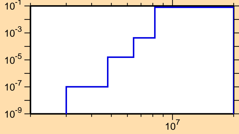
\sigma vs. E for ^{83}\text{Zr}(n,p\alpha)
