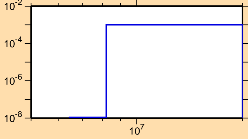
\sigma vs. E for ^{83}\text{Zr}(n,\alpha)
