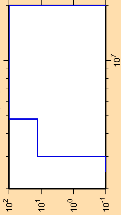
\Delta\sigma/\sigma vs. E for ^{83}\text{Zr}(n,d)
