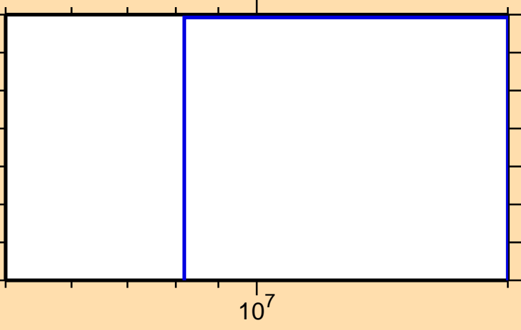
\sigma vs. E for ^{83}\text{Zr}(n,\text{pt})
