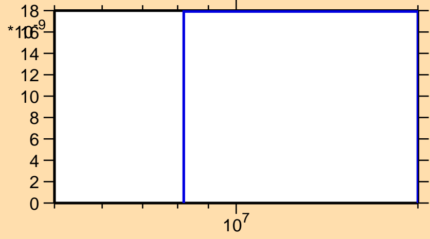
\sigma vs. E for ^{83}\text{Zr}(n,\text{nd})
