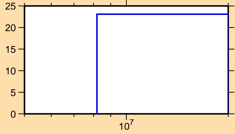
\Delta\sigma/\sigma vs. E for ^{83}\text{Zr}(n,\text{el.})
