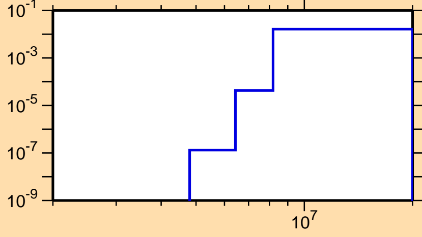
\sigma vs. E for ^{83}\text{Zr}(n,d)
