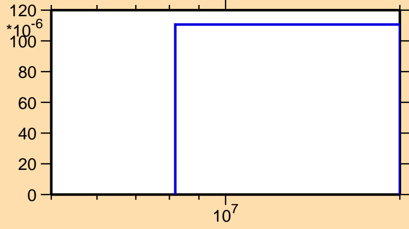
\sigma vs. E for ^{83}\text{Zr}(n,t)
