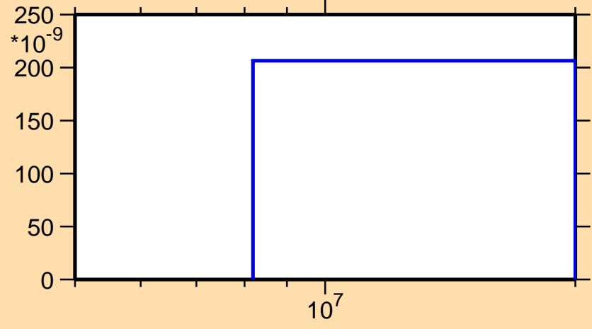
\sigma vs. E for ^{83}\text{Zr}(n,2np)
