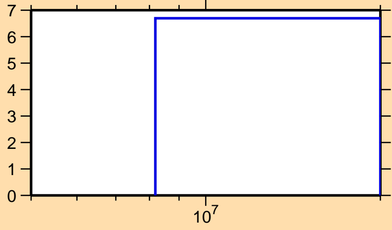
\Delta\sigma/\sigma vs. E for ^{83}\text{Zr}(n,\text{nonel.})
