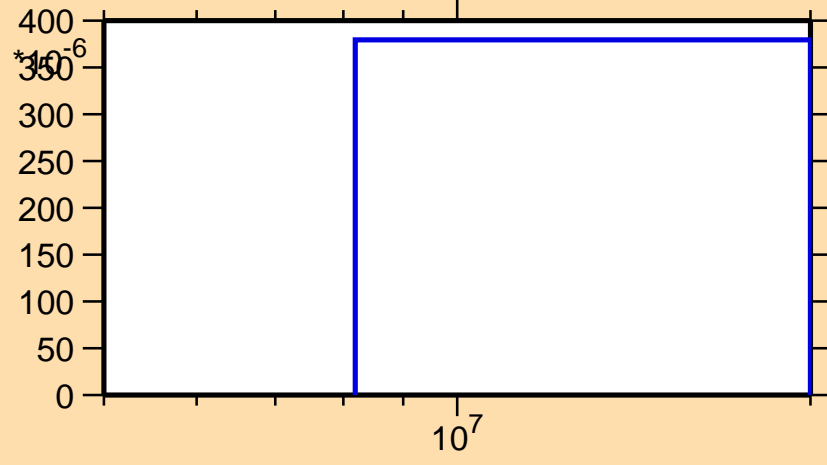
\sigma vs. E for ^{83}\text{Zr}(n,pd)
