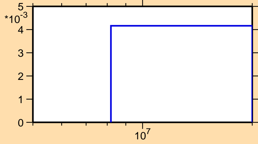
\sigma vs. E for ^{83}\text{Zr}(n,2n)
