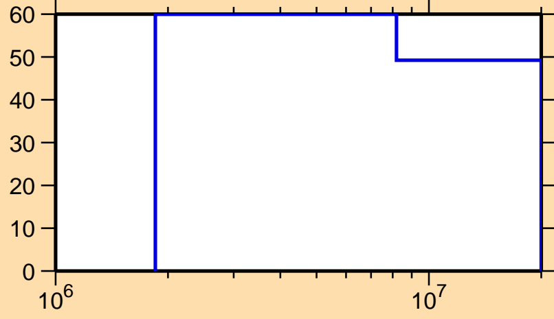
\Delta\sigma/\sigma vs. E for ^{83}\text{Zr}(n,n\text{cont.})
