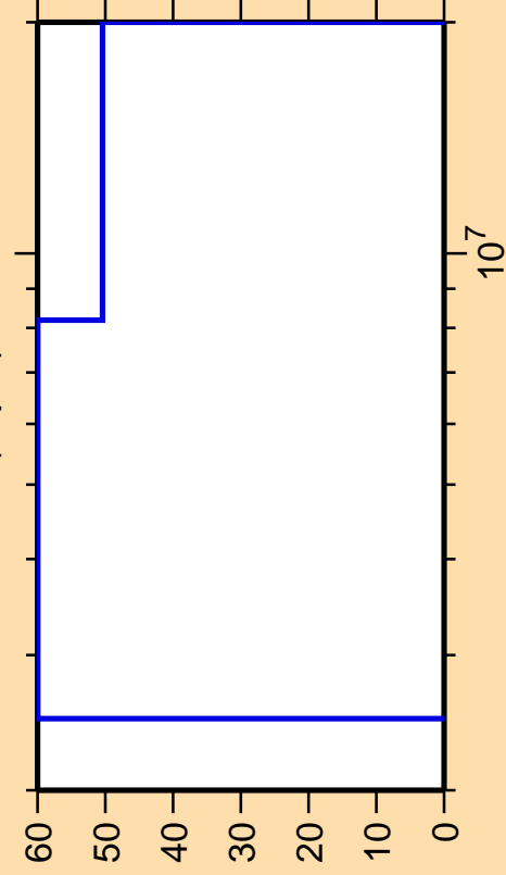
\Delta\sigma/\sigma vs. E for ^{83}\text{Zr}(n,p\alpha)
