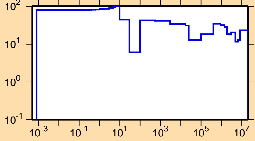
\Delta\sigma/\sigma vs. E for ^{83}\text{Zr}(n,el.)
