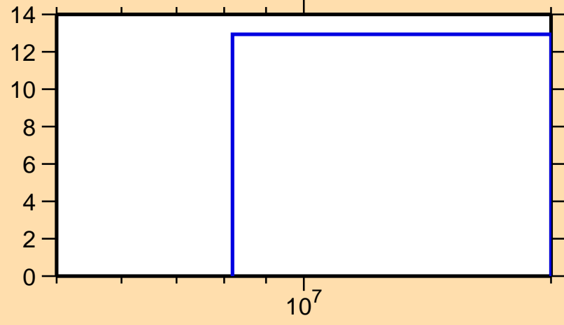
\Delta\sigma/\sigma vs. E for ^{83}\text{Zr}(n,\text{tot.})
