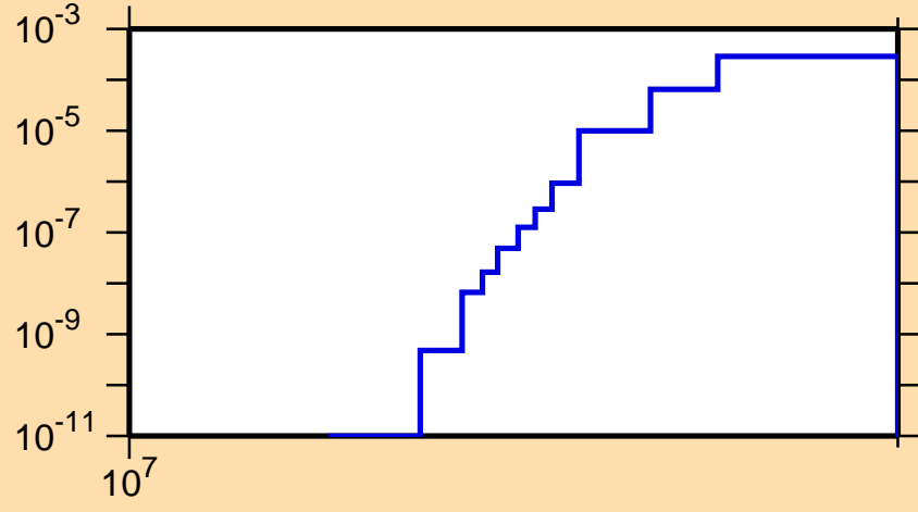
\sigma vs. E for ^{84}\text{Zr}(n,t)
