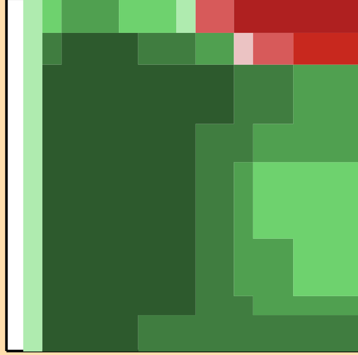
\Delta\sigma/\sigma vs. E for ^{84}\text{Zr}(n,n\text{cont.})
