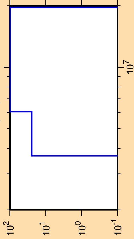
\Delta\sigma/\sigma vs. E for ^{84}\text{Zr}(n,d)
