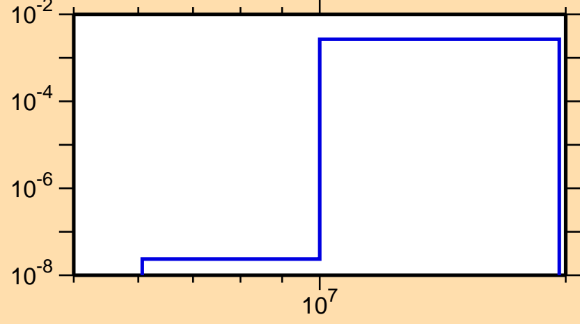
\sigma vs. E for ^{84}\text{Zr}(n,p\alpha)
