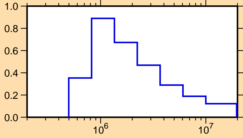
\sigma vs. E for ^{84}\text{Zr}(n,n_1)
