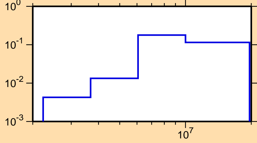
\sigma vs. E for ^{84}\text{Zr}(n,n\text{cont.})
