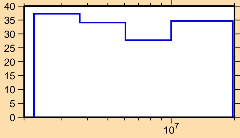
\Delta\sigma/\sigma vs. E for ^{84}\text{Zr}(n,inel.)
