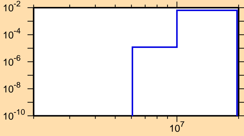
\sigma vs. E for ^{84}\text{Zr}(n,d)
