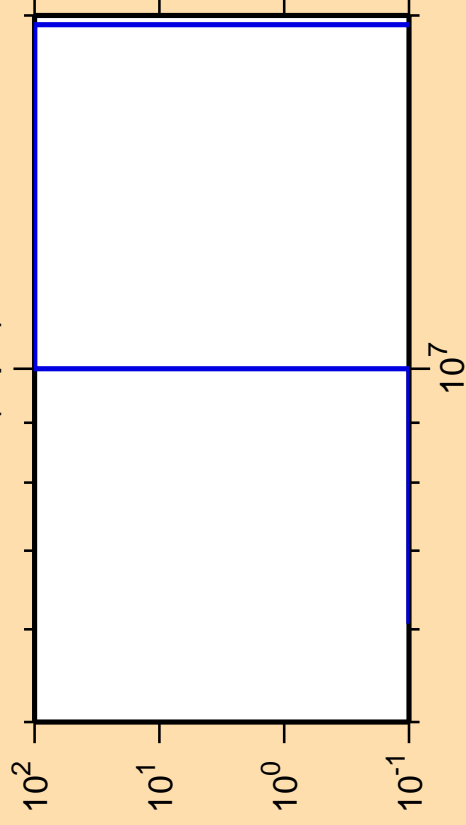
\Delta\sigma/\sigma vs. E for ^{84}\text{Zr}(n,pd)
