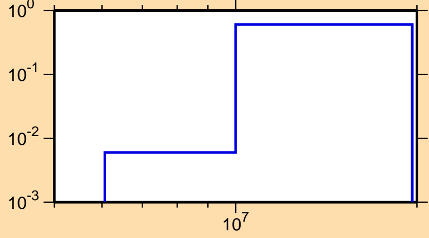
\sigma vs. E for ^{84}\text{Zr}(n,np)
