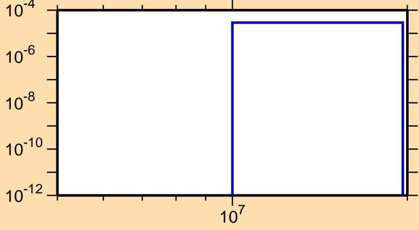
\sigma vs. E for ^{84}\text{Zr}(n,pd)
