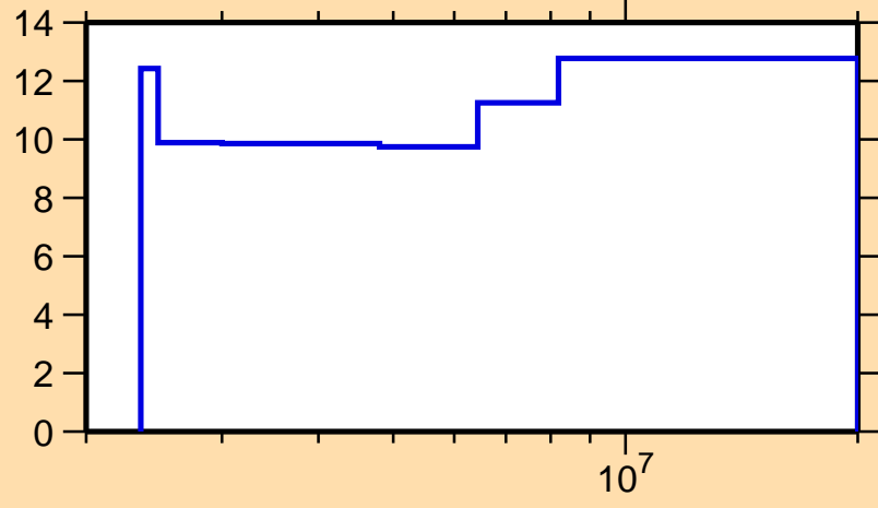
\Delta\sigma/\sigma vs. E for ^{84}\text{Zr}(n,nonel.)
