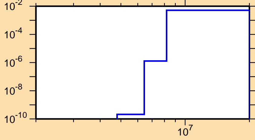
\sigma vs. E for ^{84}\text{Zr}(n,d)
