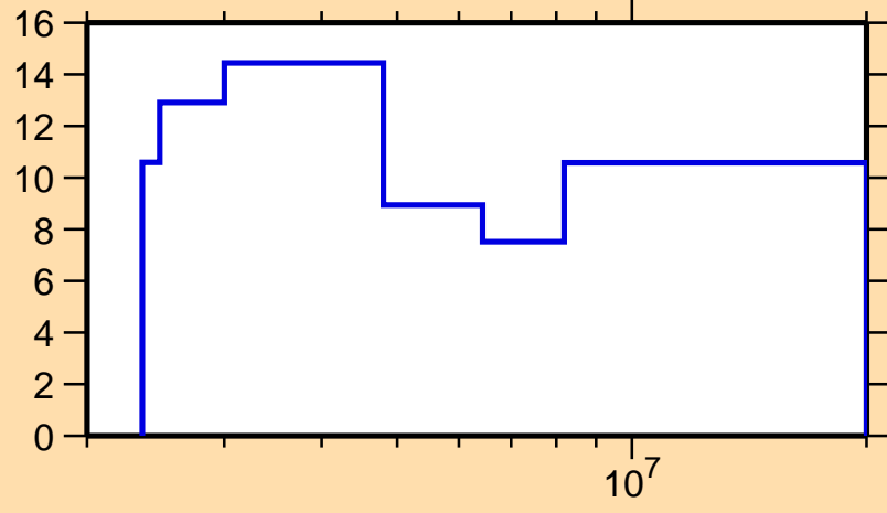
\Delta\sigma/\sigma vs. E for ^{84}\text{Zr}(n,tot.)
