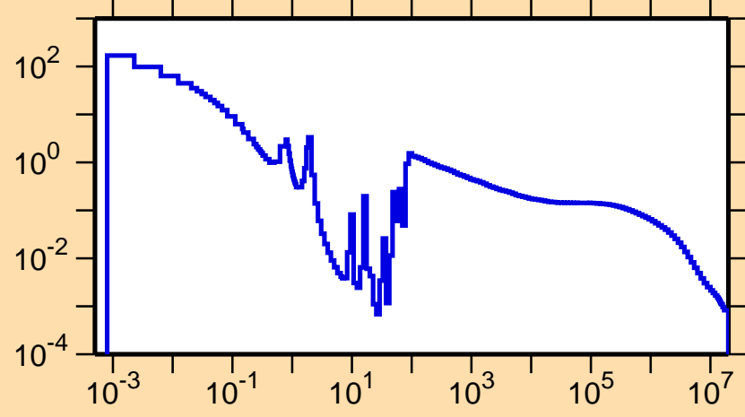
\sigma vs. E for ^{85}\text{Zr}(n,\gamma)
