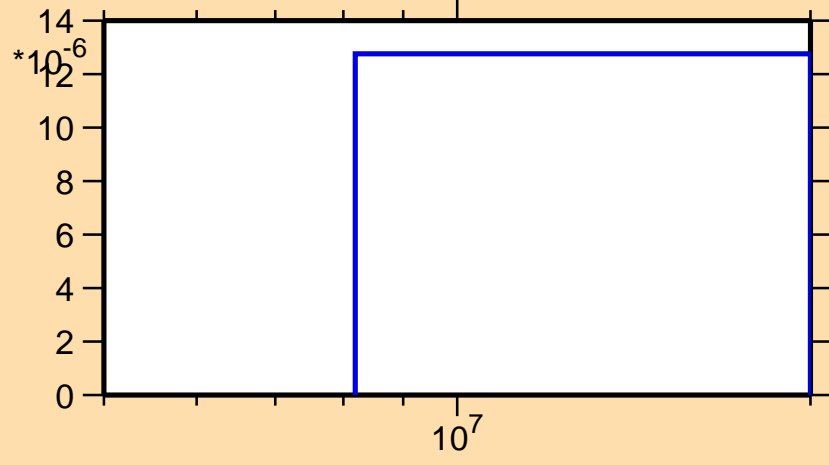
\sigma vs. E for ^{85}\text{Zr}(n,pd)
