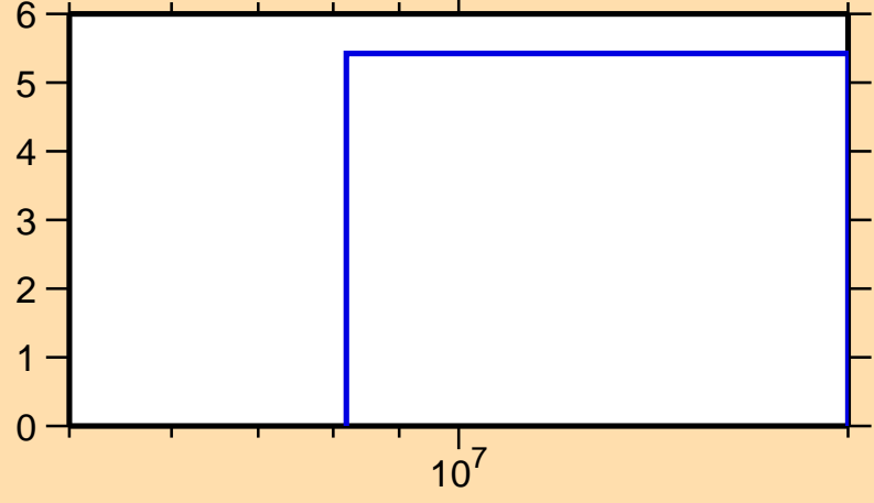
\Delta\sigma/\sigma vs. E for ^{85}\text{Zr}(n,\text{nonel.})
