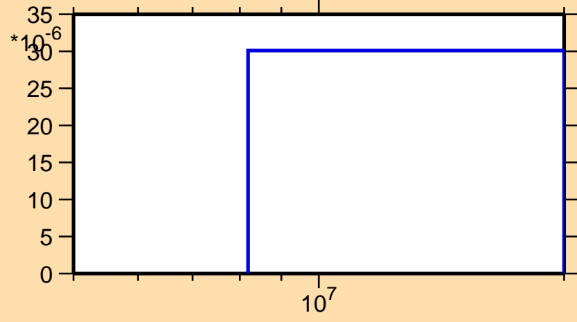
\sigma vs. E for ^{85}\text{Zr}(n,t)
