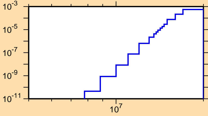
\sigma vs. E for ^{85}\text{Zr}(n,\text{He}3)
