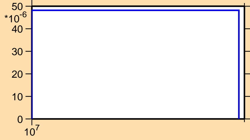
\sigma vs. E for ^{85}\text{Zr}(n,pd)
