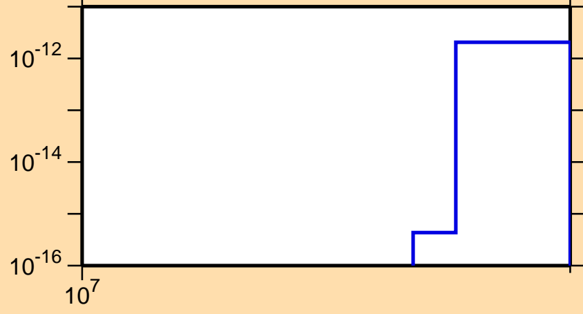
\sigma vs. E for ^{86}\text{Zr}(\text{mt117})
