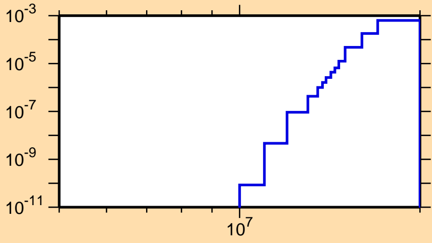
\sigma vs. E for ^{86}\text{Zr}(n,p\alpha)
