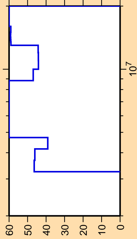
\Delta\sigma/\sigma vs. E for ^{86}\text{Zr}(n,p)
