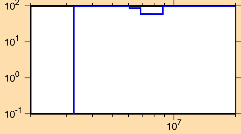
\Delta\sigma/\sigma vs. E for ^{86}\text{Zr}(n,n\text{cont.})
