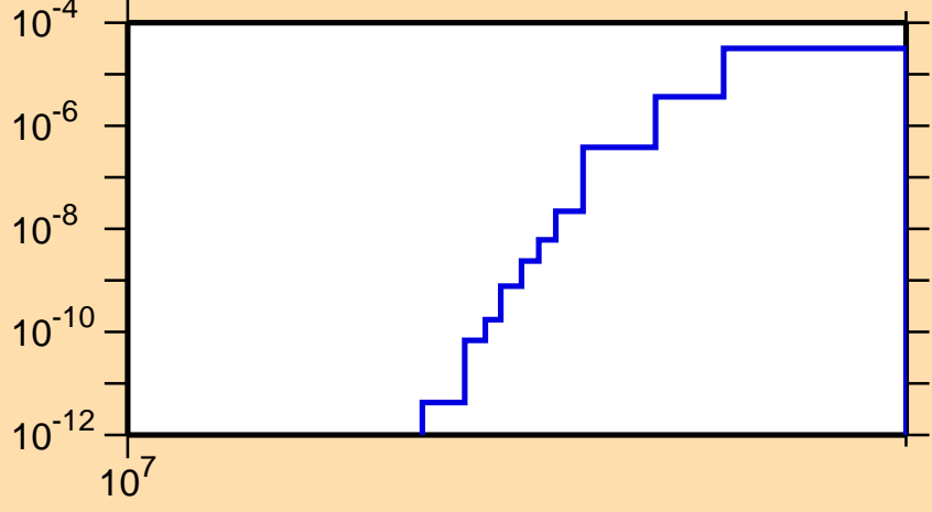
\sigma vs. E for ^{86}\text{Zr}(n,pd)
