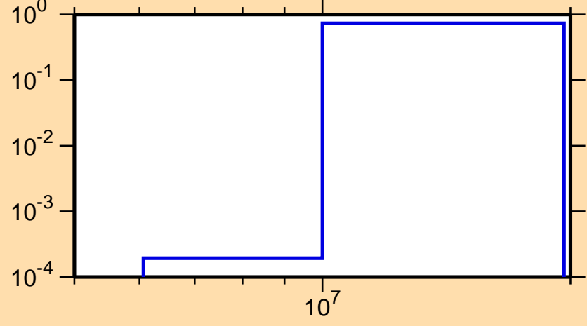
\sigma vs. E for ^{86}\text{Zr}(n,np)
