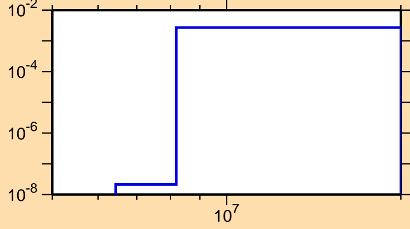
\sigma vs. E for ^{86}\text{Zr}(n,d)
