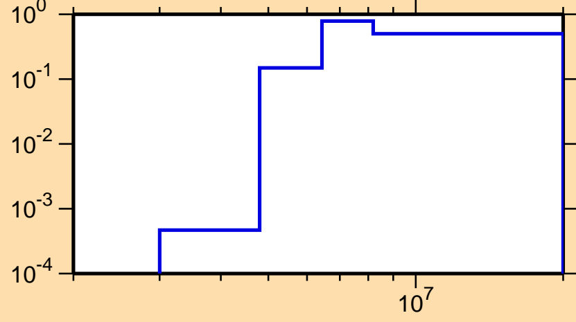
\sigma vs. E for ^{86}\text{Zr}(n,n\text{cont.})
