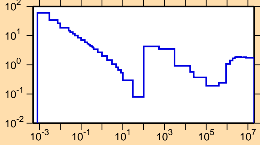
\sigma vs. E for ^{86}\text{Zr}(n,\text{nonel.})
