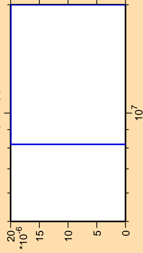
\Delta\sigma/\sigma vs. E for ^{86}\text{Zr}(n,2np)
