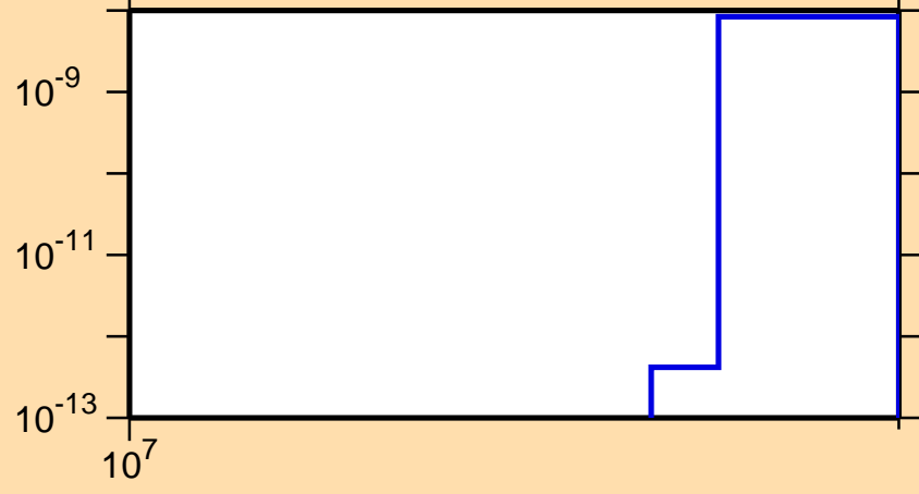
\sigma vs. E for ^{87}\text{Zr}(n,\text{pt})
