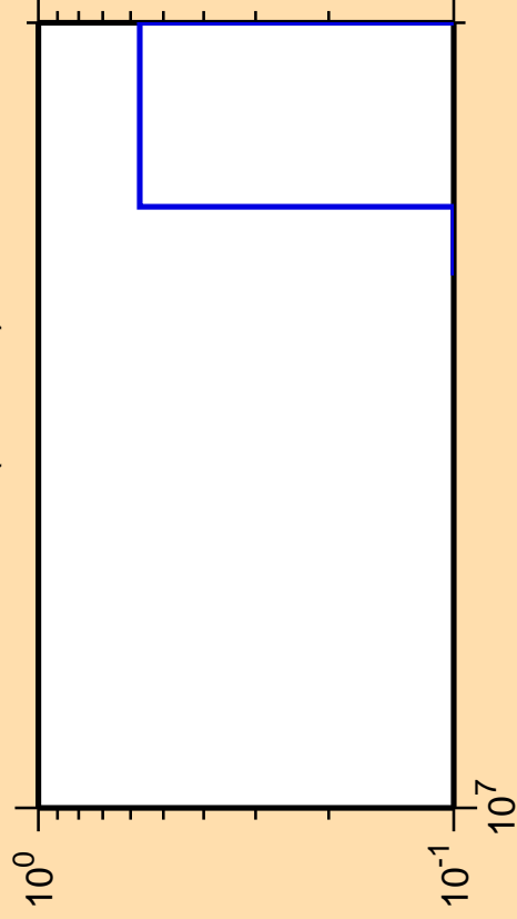
\Delta\sigma/\sigma vs. E for ^{87}\text{Zr}(\text{mt117})
