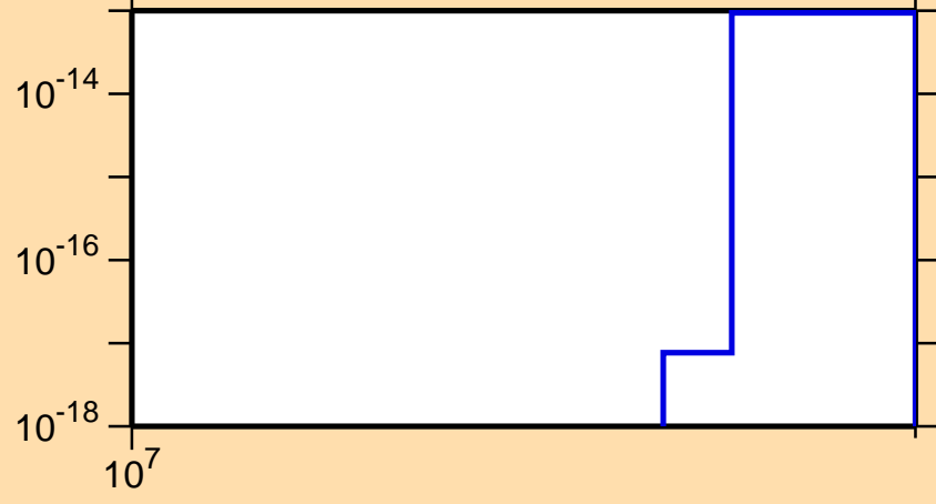
\sigma vs. E for ^{87}\text{Zr}(\text{mt117})
