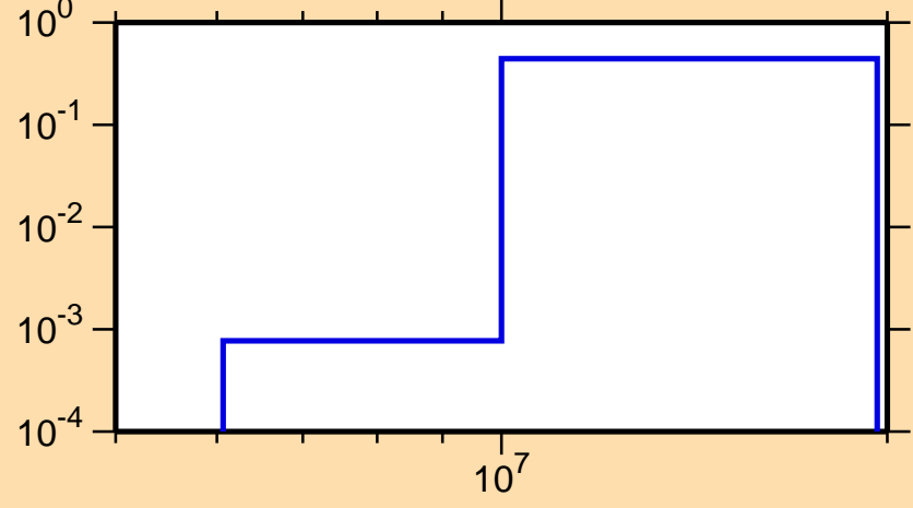
\sigma vs. E for ^{87}\text{Zr}(n,np)
