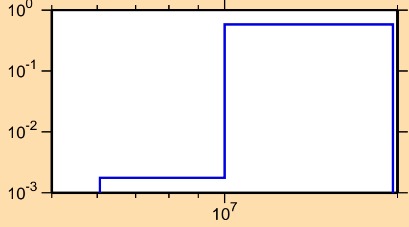
\sigma vs. E for ^{87}\text{Zr}(n,2n)
