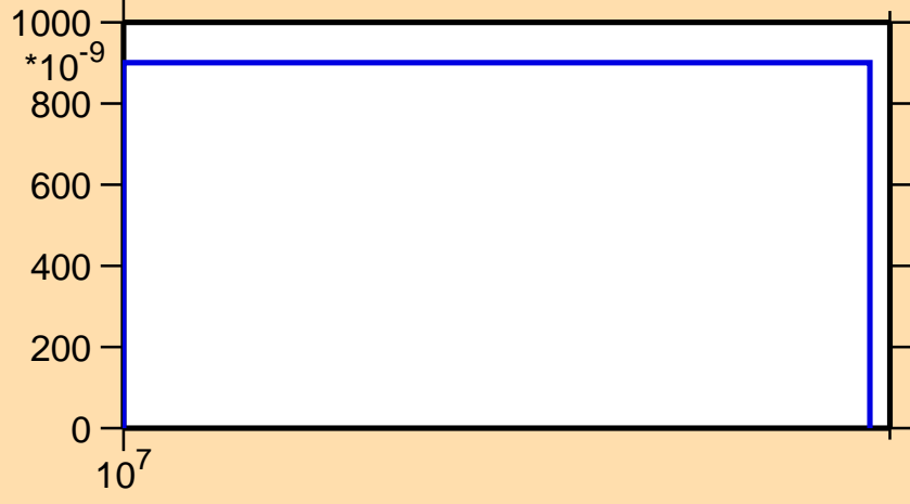
\sigma vs. E for ^{87}\text{Zr}(n,pd)
