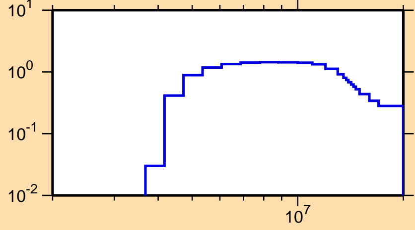
\sigma vs. E for ^{88}\text{Zr}(n,n\text{cont.})
