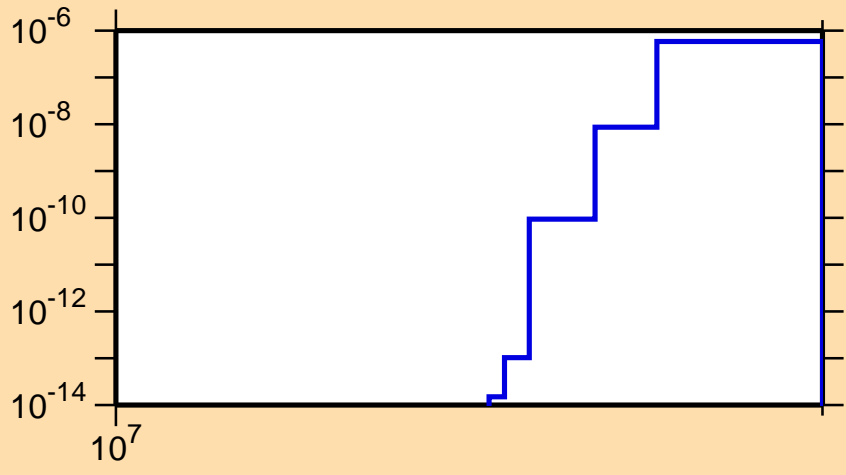
\sigma vs. E for ^{88}\text{Zr}(n,pd)
