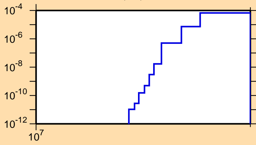
\sigma vs. E for ^{88}\text{Zr}(n,t)
