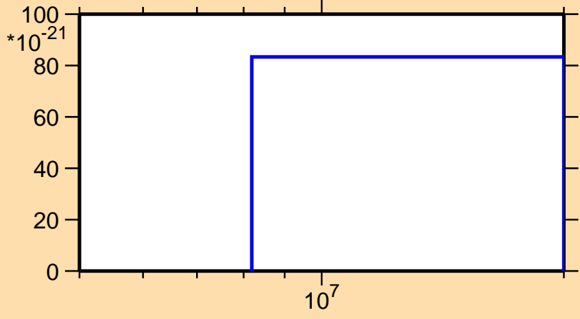
\sigma vs. E for ^{88}\text{Zr}(n,2np)
