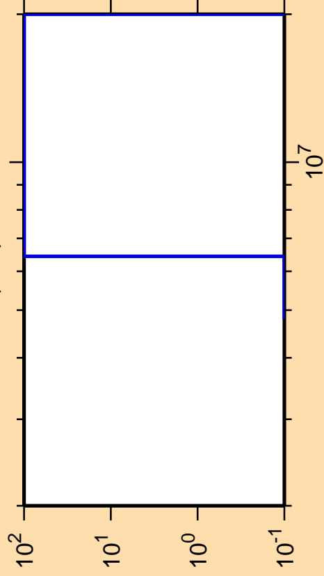
\Delta\sigma/\sigma vs. E for ^{88}\text{Zr}(n,d)
