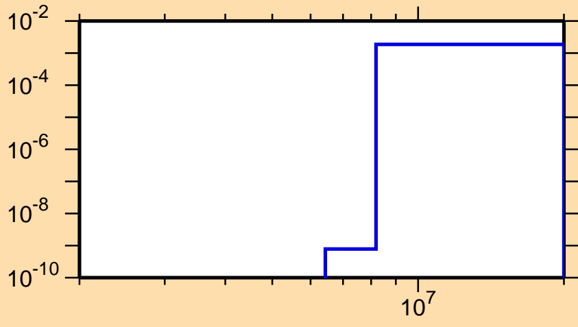
\sigma vs. E for ^{88}\text{Zr}(n,d)
