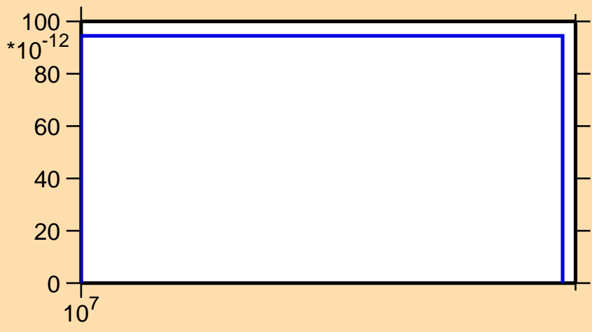
\sigma vs. E for ^{90}\text{Zr}(n,pd)
