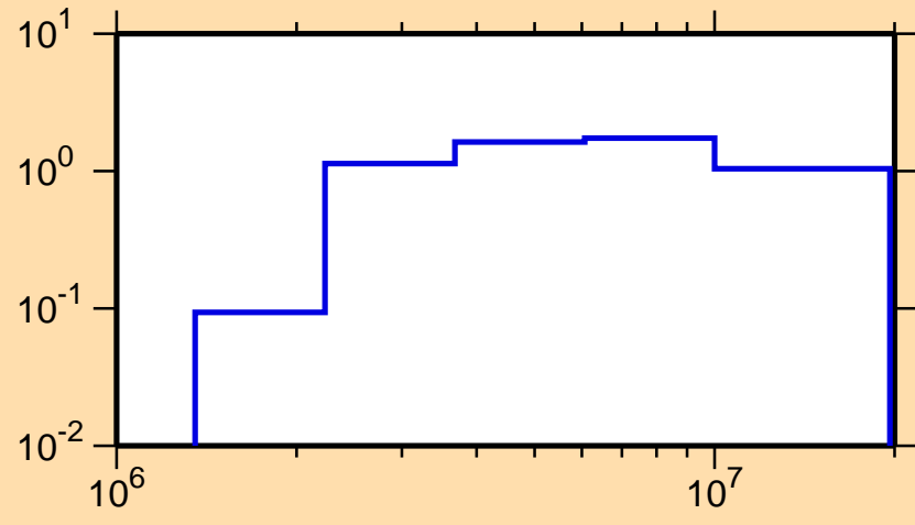
\sigma vs. E for ^{90}\text{Zr}(n,\text{inel.})
