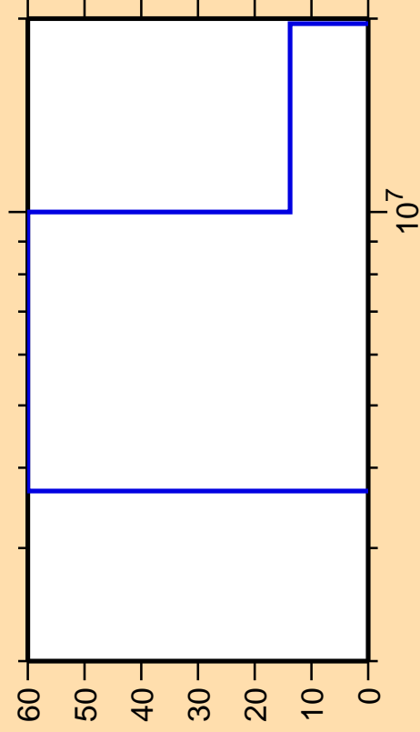
\Delta\sigma/\sigma vs. E for ^{90}\text{Zr}(n,\alpha)
