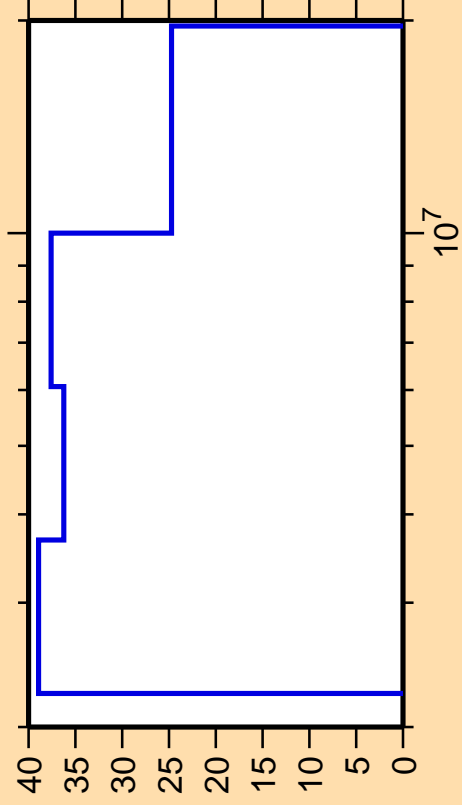
\Delta\sigma/\sigma vs. E for ^{90}\text{Zr}(n,n_3)
