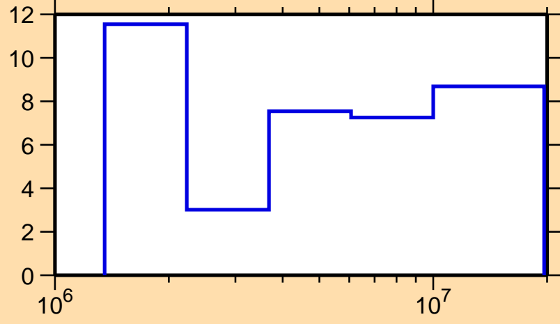
\Delta\sigma/\sigma vs. E for ^{90}\text{Zr}(n,el.)
