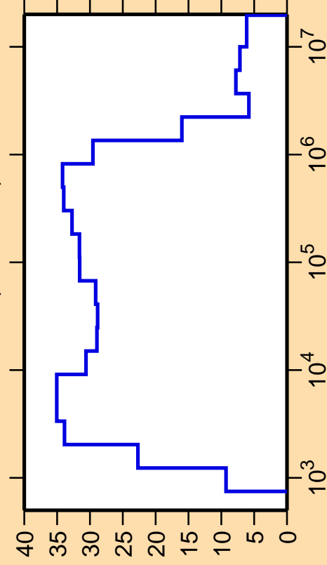
\Delta\sigma/\sigma vs. E for ^{90}\text{Zr}(n,\text{nonel.})
