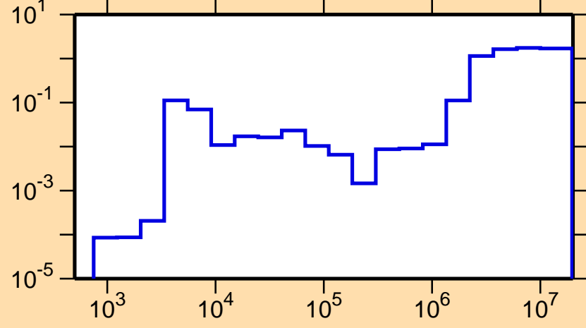
\sigma vs. E for ^{90}\text{Zr}(n,\text{nonel.})
