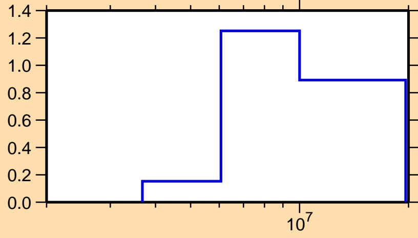
\sigma vs. E for ^{90}\text{Zr}(n,n\text{cont.})
