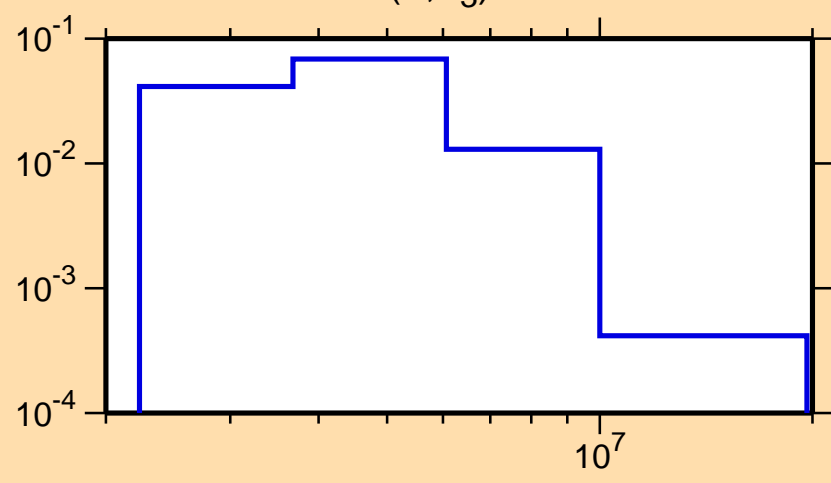
\sigma vs. E for ^{90}\text{Zr}(n,n_3)
